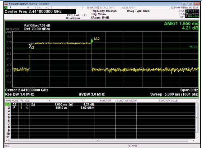
8DPSK / 3-DH3
