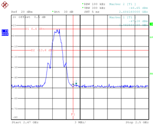
BLE: Band edge-right side
