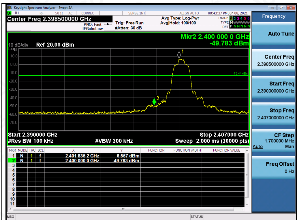
Test Graph EDR ANT1 2402 2Mbps Lower Band Edge Emissions
