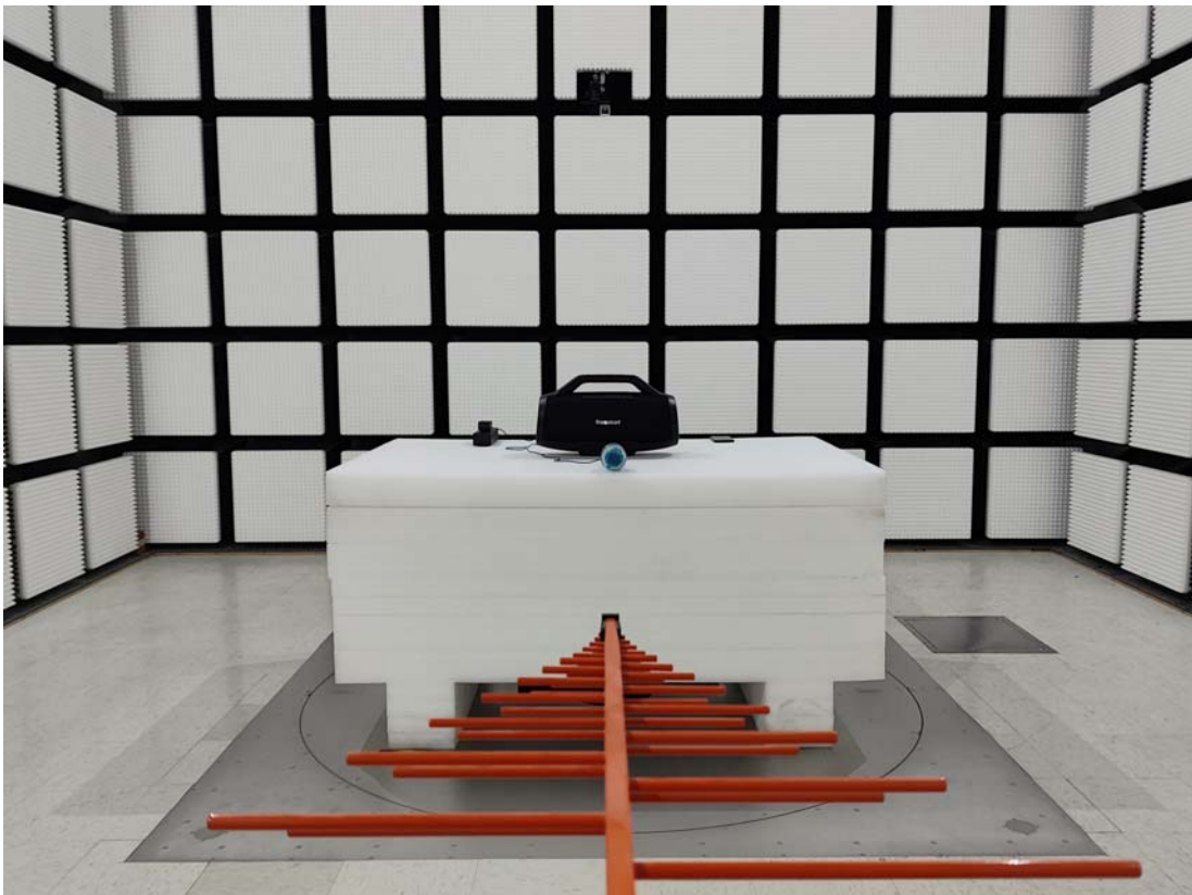
Radiated Emission Below 1GHz View- Adapter#2
