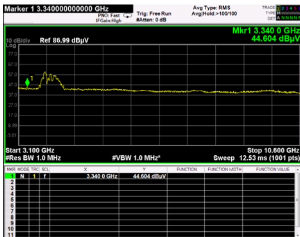
Horizontal(3 100-10 600 MHz)
