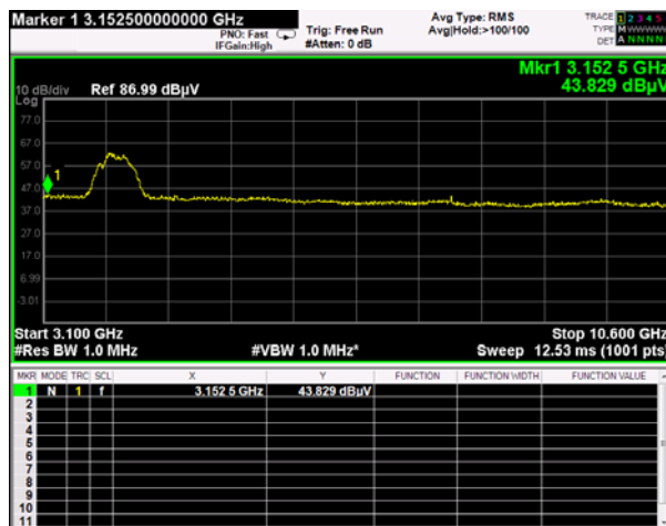
Vertical(3 100-10 600 MHz)
