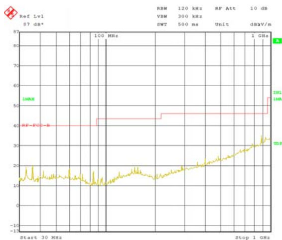
Horizontal
