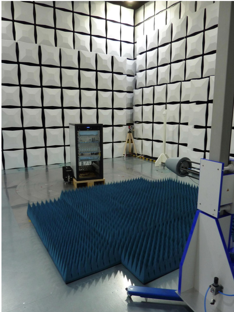
Test setup semi anechoic chamber 1 GHz – 12 GHz
