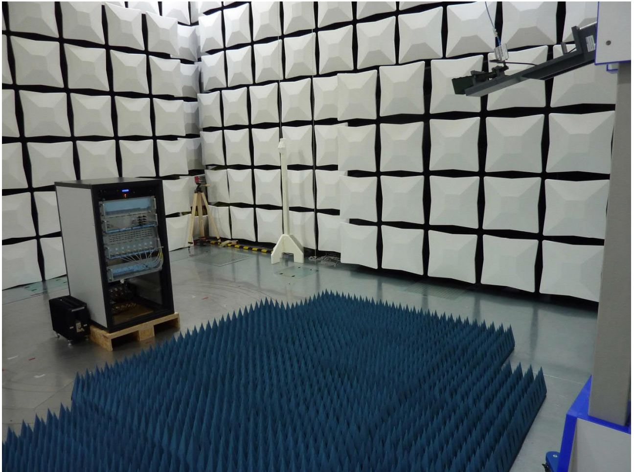
Test setup semi anechoic chamber 12 GHz – 18 GHz
