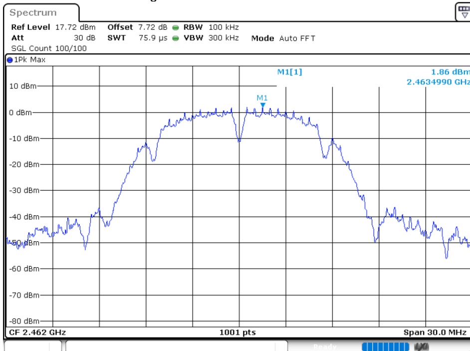
Band Edge NVNT 802.11b 2462MHz Ant1 Emission
