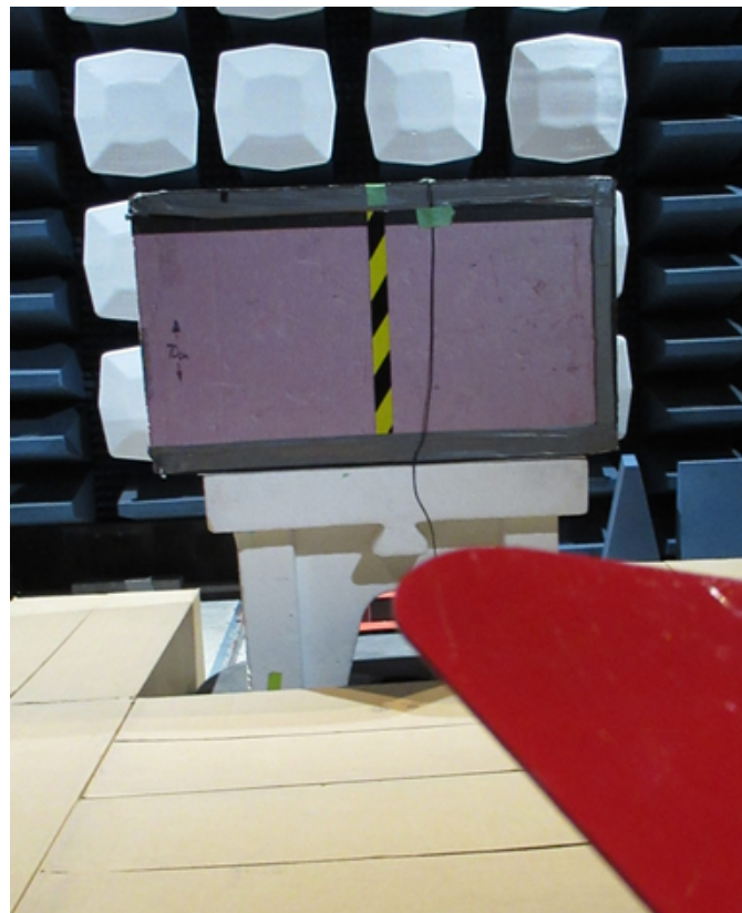
Figure 2: Radiated Emissions above 1GHz
