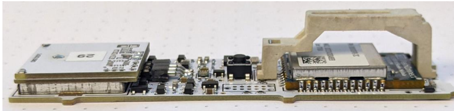
Back
