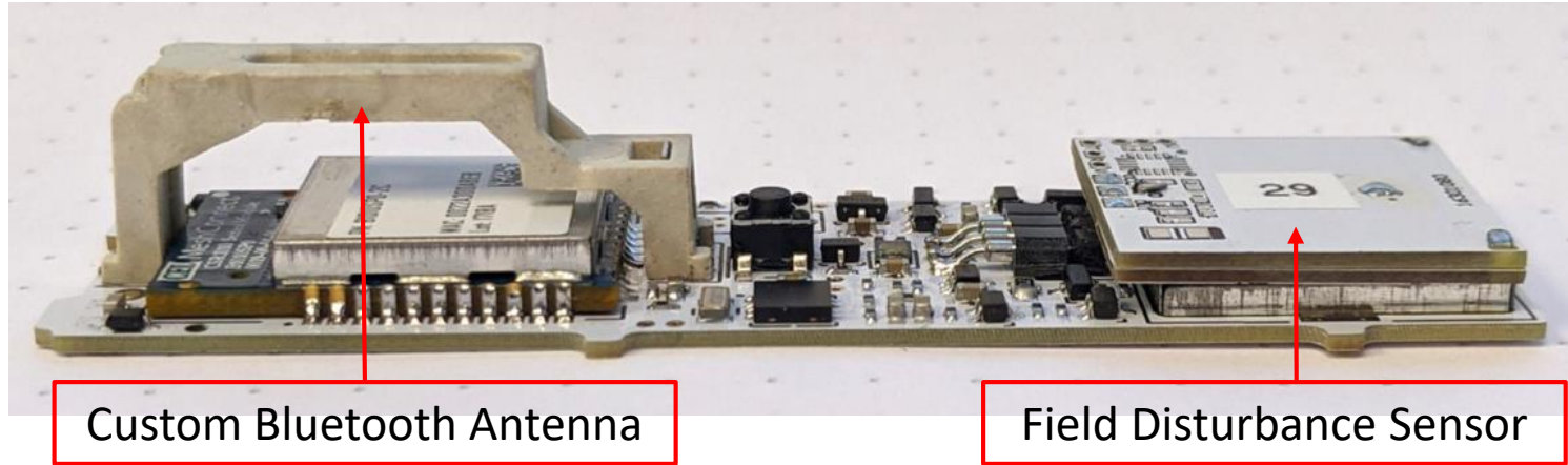
Front
