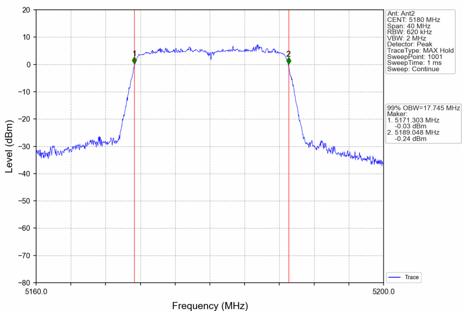
802.11ac(VHT20)_LCH_5180MHz_Ant2_NTNV_SISO
