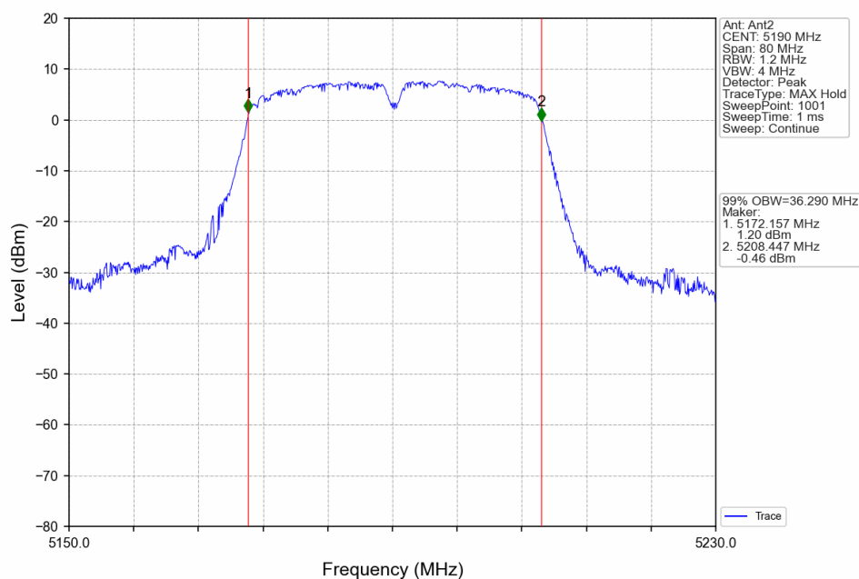
802.11ac(VHT40)_LCH_5190MHz_Ant2_NTNV_SISO
