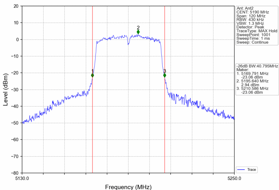
802.11n(HT40)_LCH_5190MHz_Ant2_NTNV_MIMO
