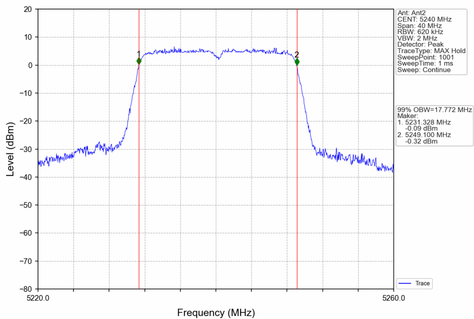
802.11n(HT20)_HCH_5240MHz_Ant2_NTNV_MIMO
