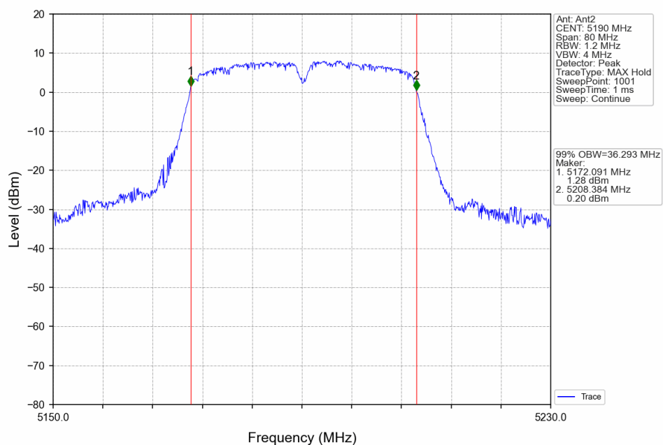
802.11ac(VHT40)_LCH_5190MHz_Ant2_NTNV_MIMO
