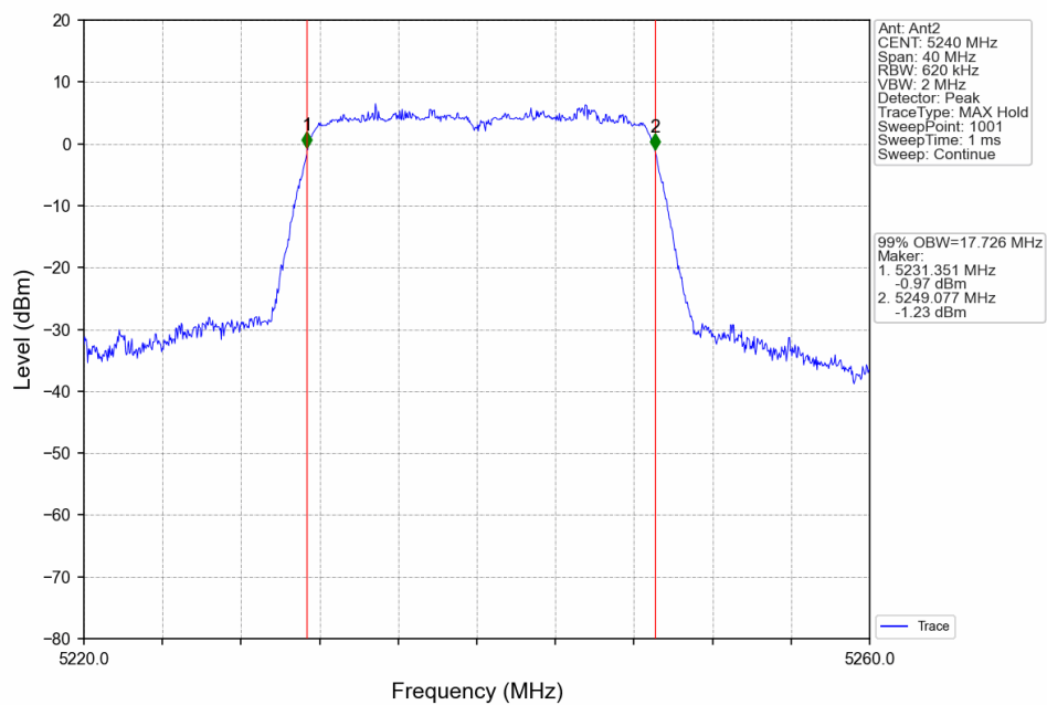
802.11ac(VHT20)_HCH_5240MHz_Ant2_NTNV_MIMO
