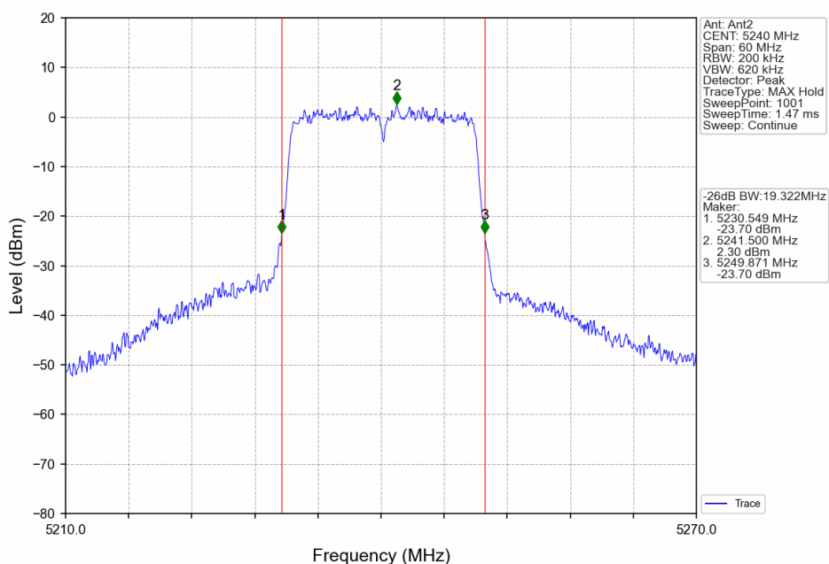
802.11n(HT20)_HCH_5240MHz_Ant2_NTNV_SISO
