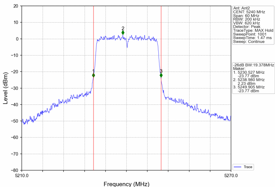
802.11n(HT20)_HCH_5240MHz_Ant2_NTNV_MIMO
