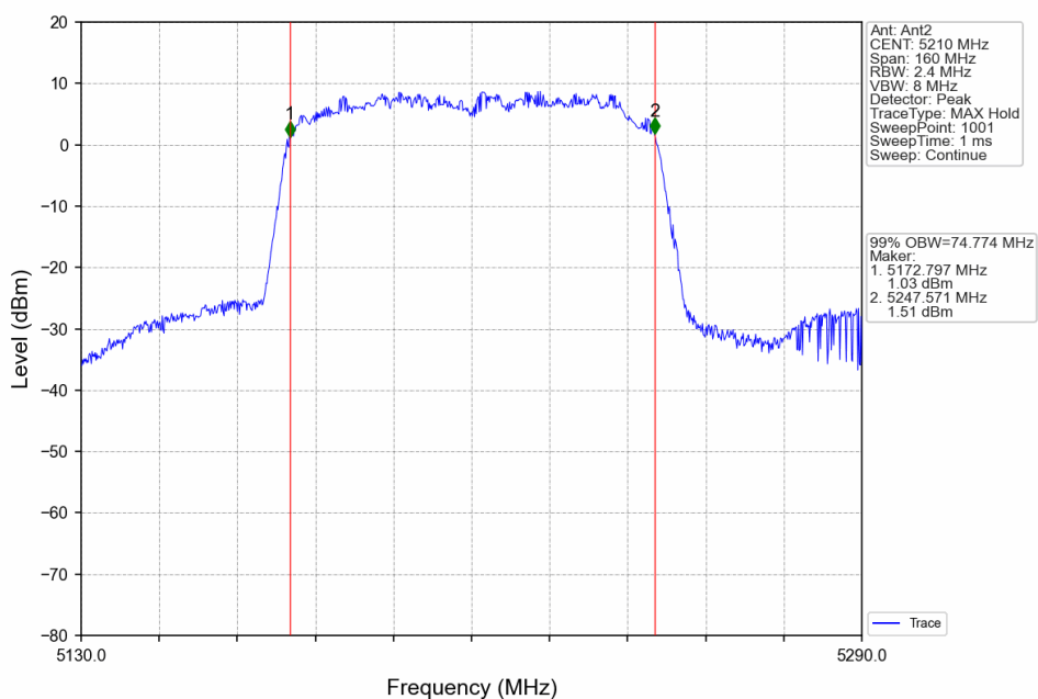
802.11ac(VHT80)_MCH_5210MHz_Ant2_NTNV_SISO
