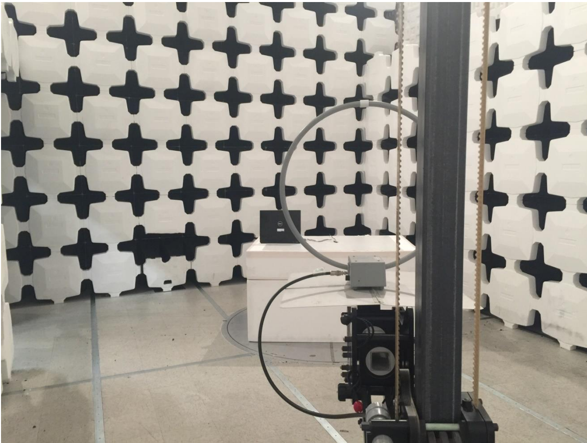
PHOTO 2. RADIATED EMISSIONS TEST SETUP – BELOW 30 MHZ
