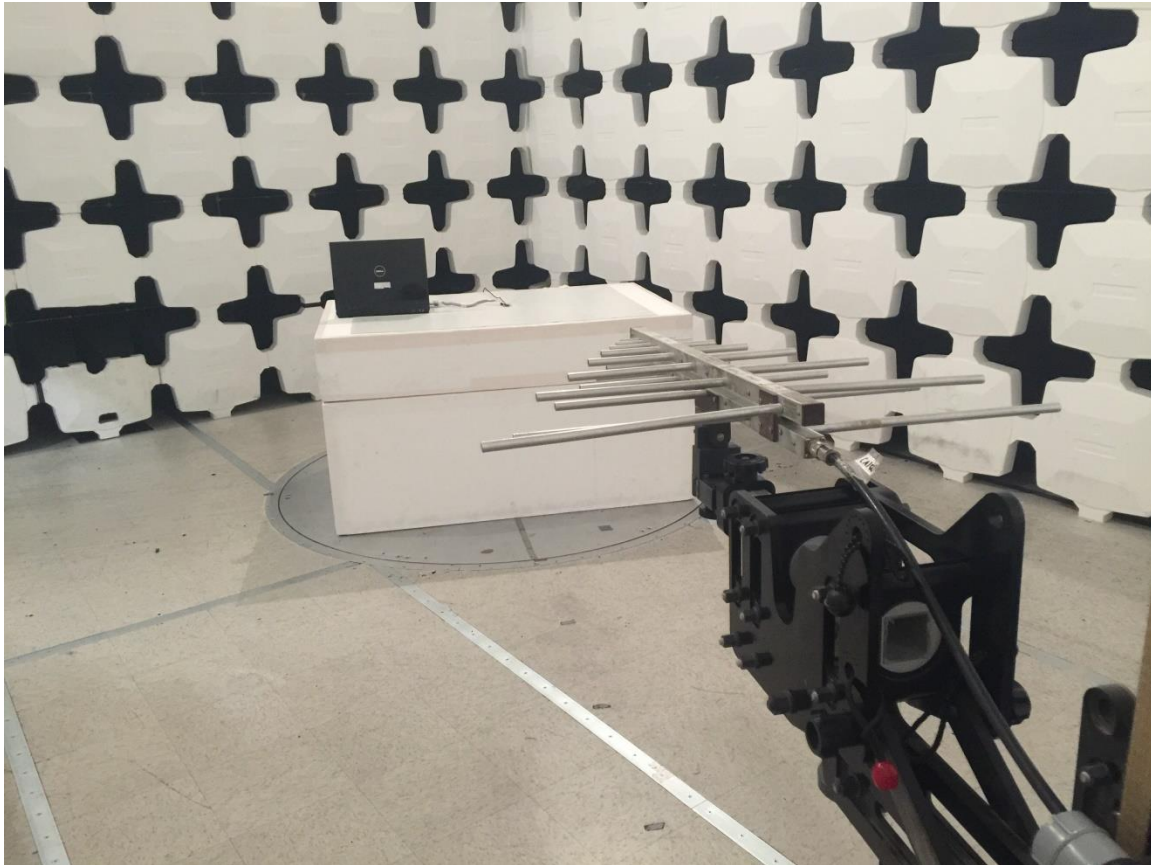
PHOTO 4. RADIATED EMISSIONS TEST SETUP – 200 TO 1000 MHZ
