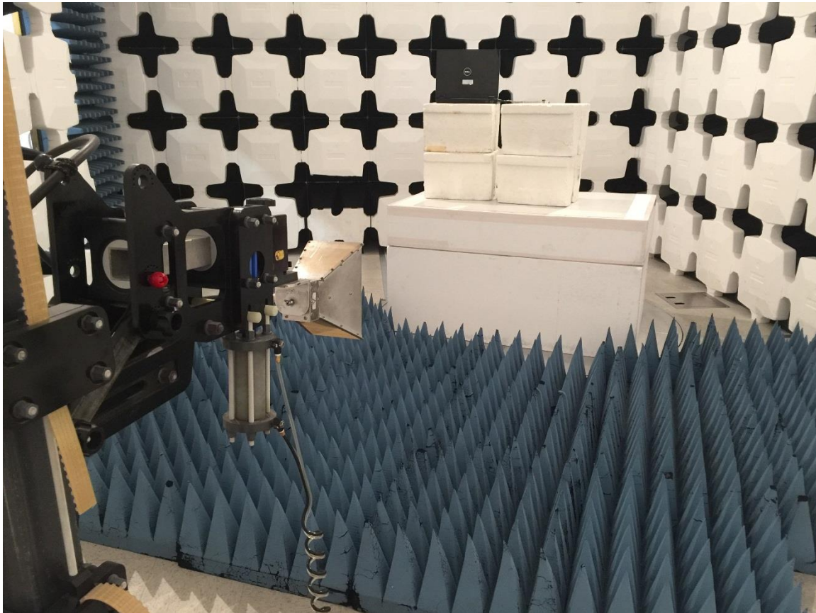
PHOTO 5. RADIATED EMISSION TEST SETUP – ABOVE 1 GHz (Intentional Spurious Emissions)
