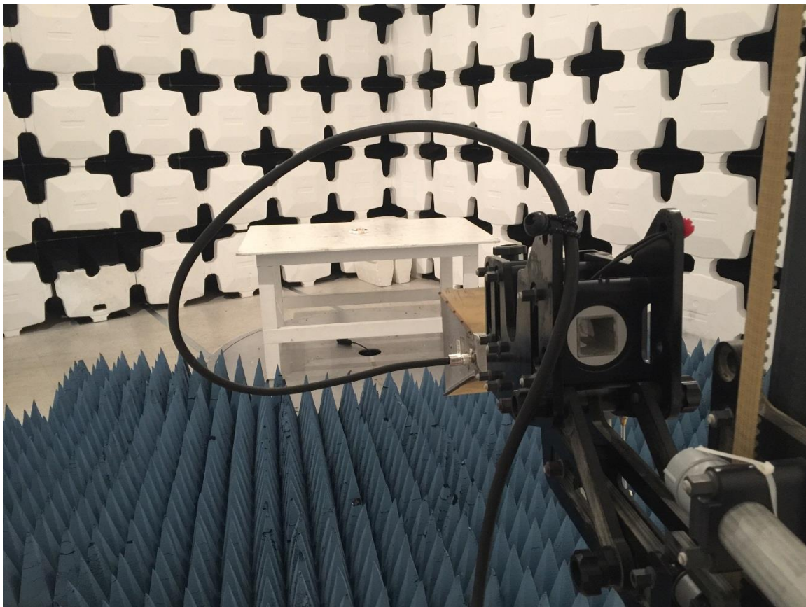
PHOTO 6. RADIATED EMISSION TEST SETUP – ABOVE 1 GHz (Unintentional Spurious Emissions)
