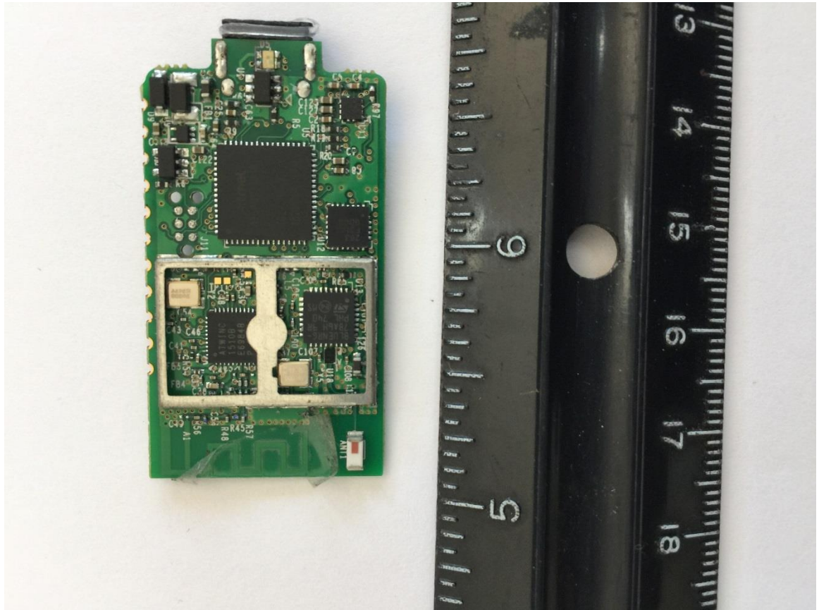
Photo 4. Module Shield Cover Removed
