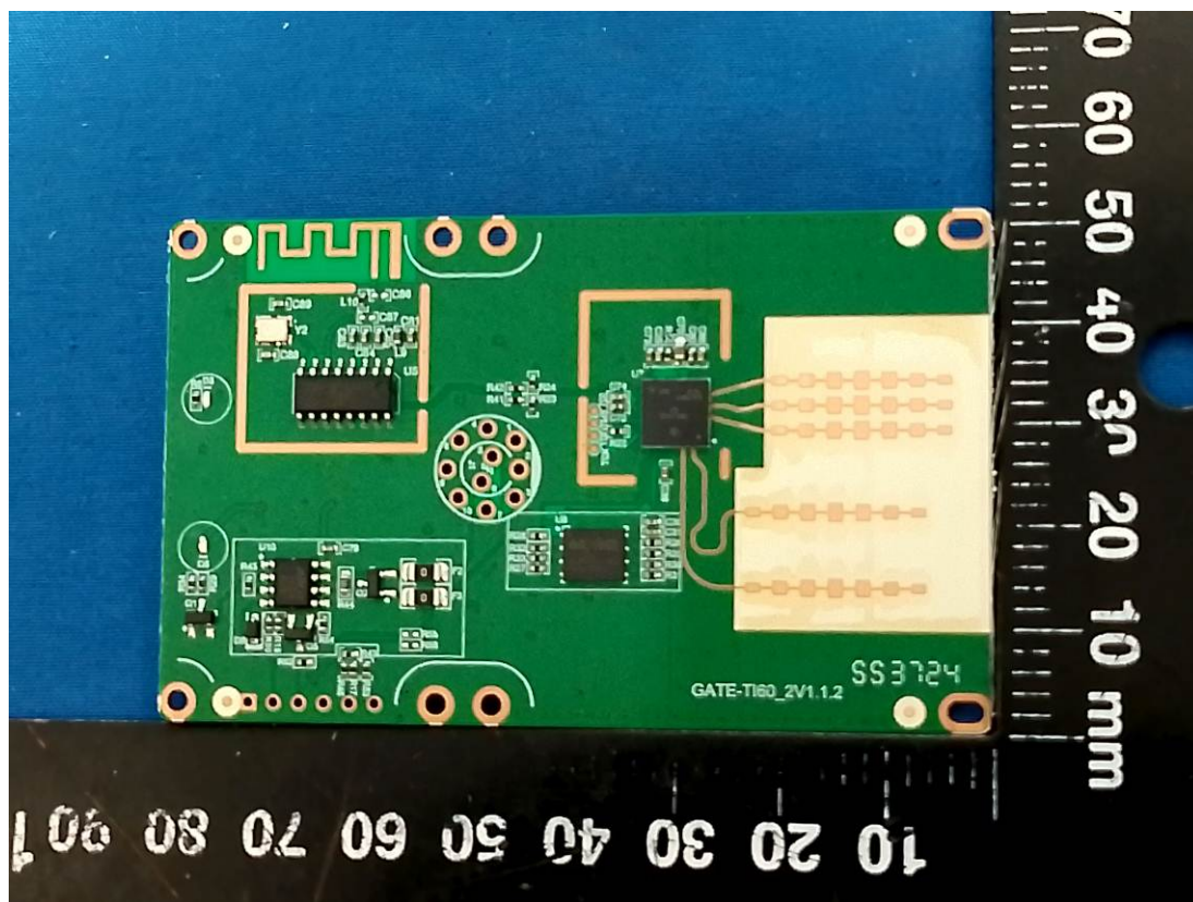
Buleetooth Chip+ Antenna
