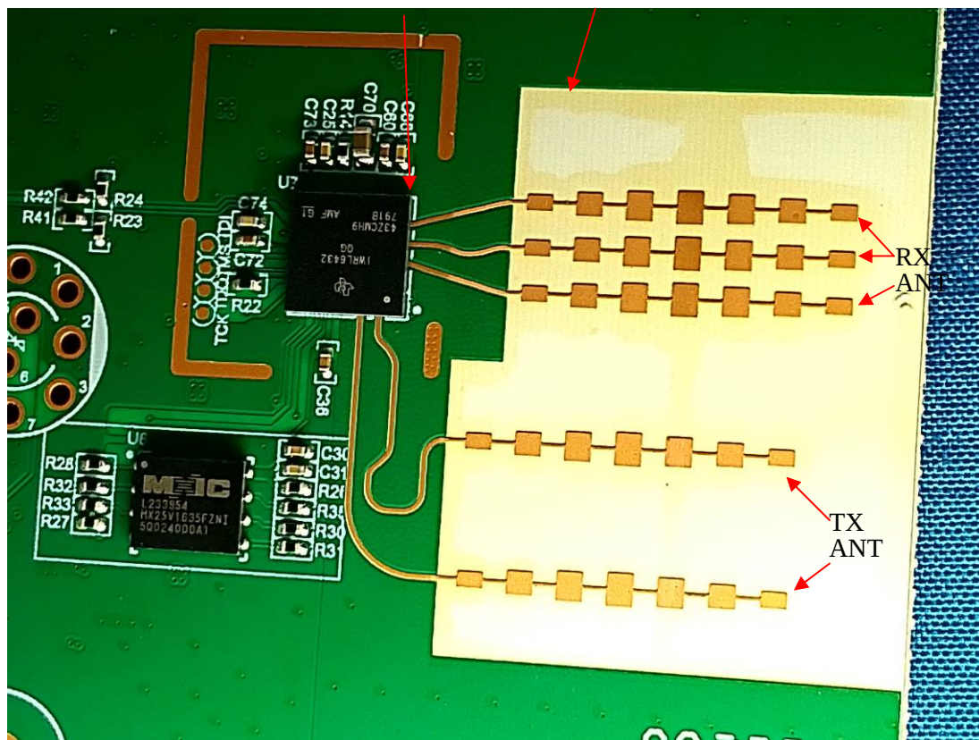
Radar Chip Radar Antenna
