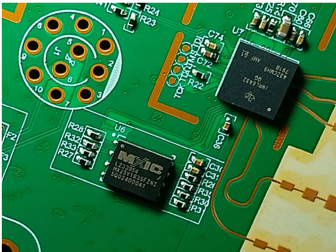
Radar Chip
