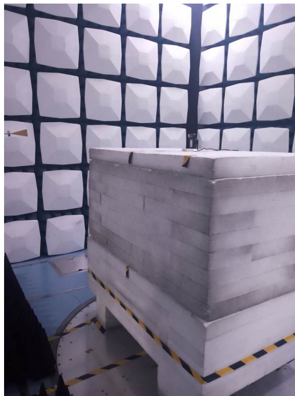
Radiated Emission 40-60GHz View
