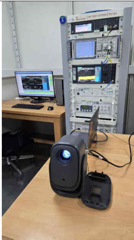
AC Power Line Conducted test
