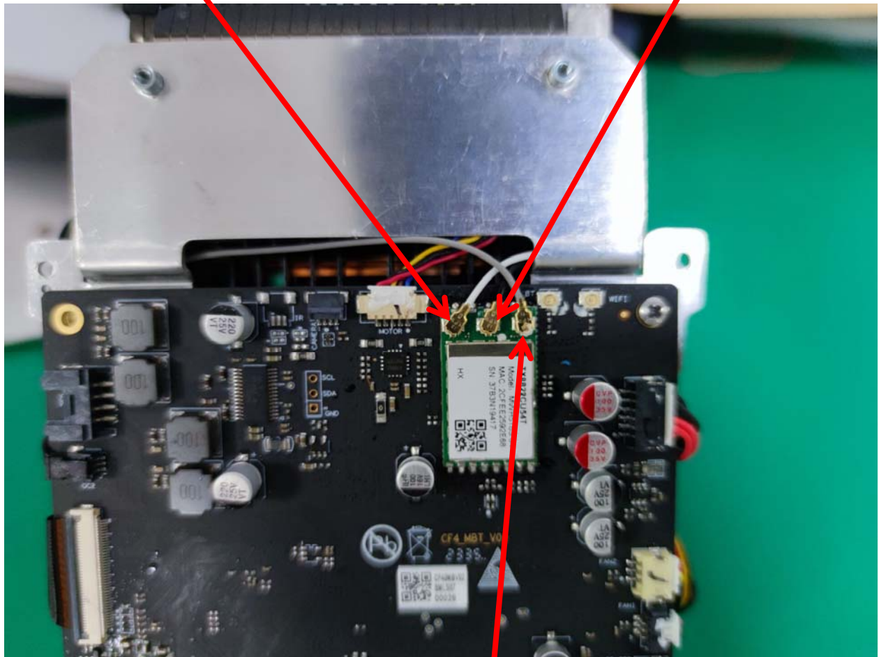
BT Antenna
