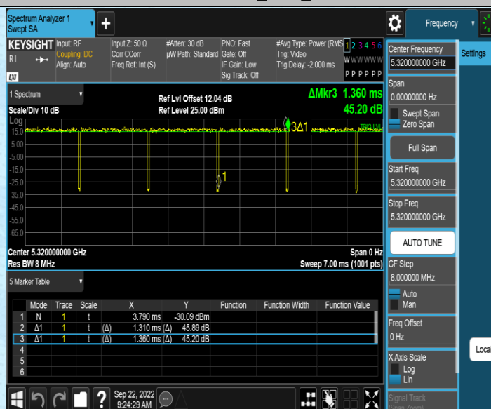
11AC20SISO_Ant2_5320
