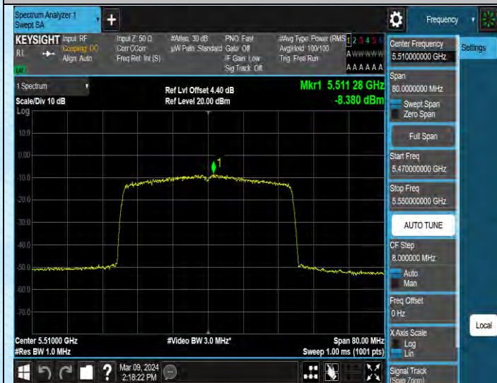
11AX40MIMO-Ant1-5510-PASS
