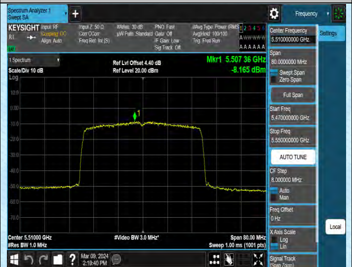
11AX40MIMO-Ant2-5510-PASS
