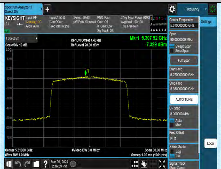
11AX40MIMO-Ant2-5310-PASS
