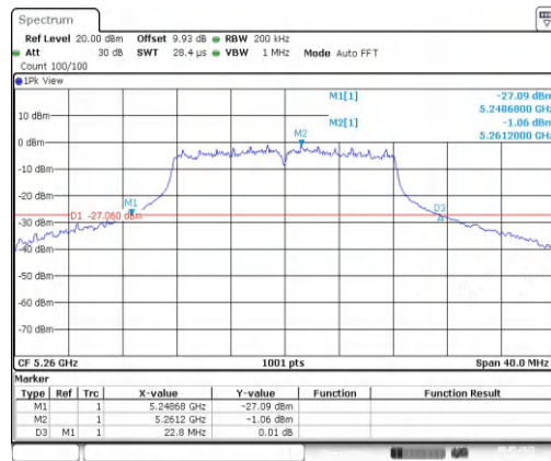
11A-CDD-Ant2-5260
