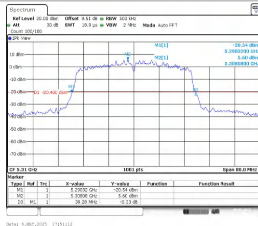
11AC40MIMO-Ant2-5310
