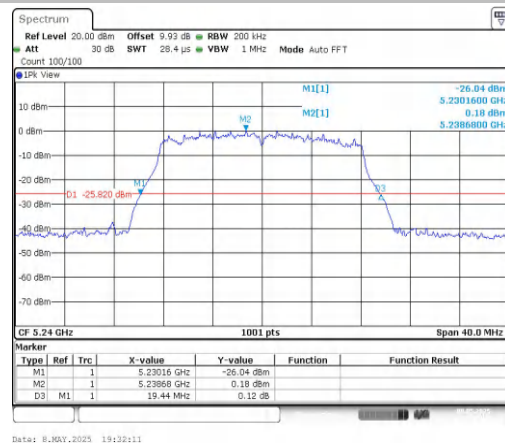
11A-CDD-Ant2-5240
