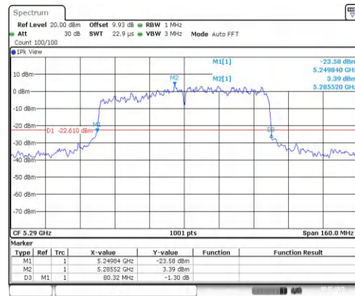
11AX80MIMO-Ant2-5290
