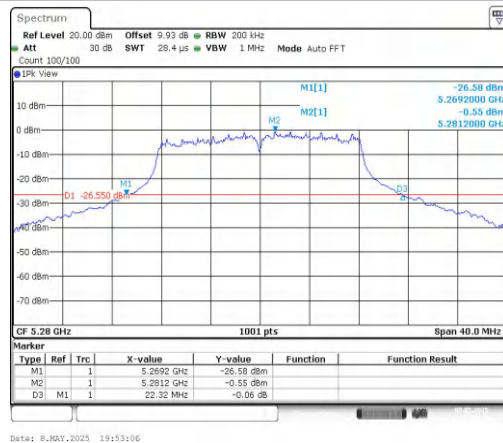
11A-CDD-Ant2-5280
