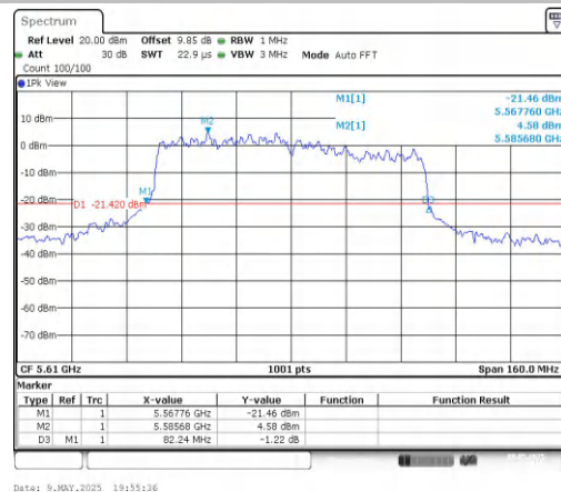
11AX80MIMO-Ant2-5610
