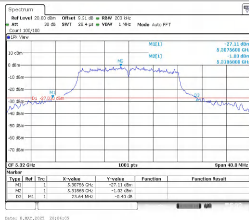
11A-CDD-Ant2-5320
