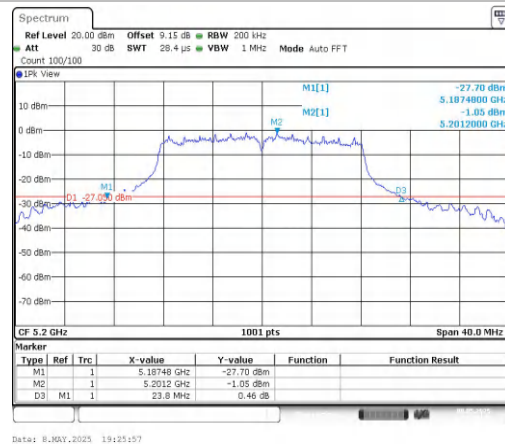
11A-CDD-Ant2-5200
