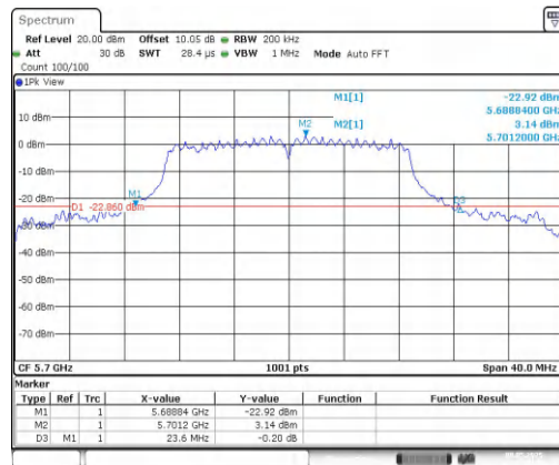
11AC20MIMO-Ant2-5700
