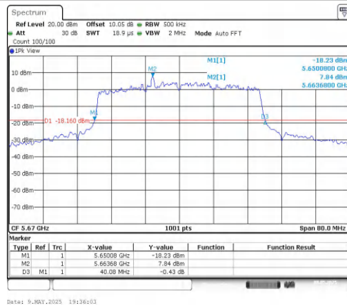
11AX40MIMO-Ant2-5670
