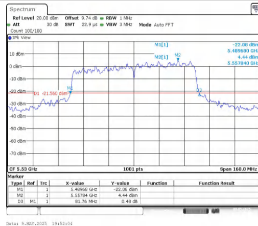
11AX80MIMO-Ant2-5530
