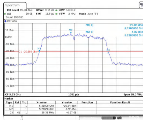
11AC40MIMO-Ant2-5230
