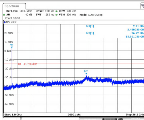
2DH5-Ant1-2480-0~Reference-PASS
