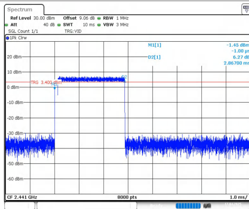
3DH3-Ant1-Hop-PASS
