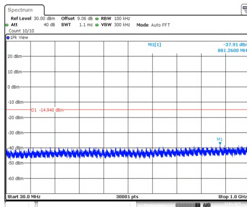
2DH5-Ant1-2441-30~1000-PASS
