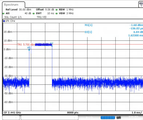
3DH1-Ant1-Hop-PASS
