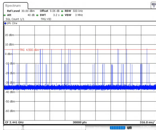
3DH1-Ant1-Hop-PASS
