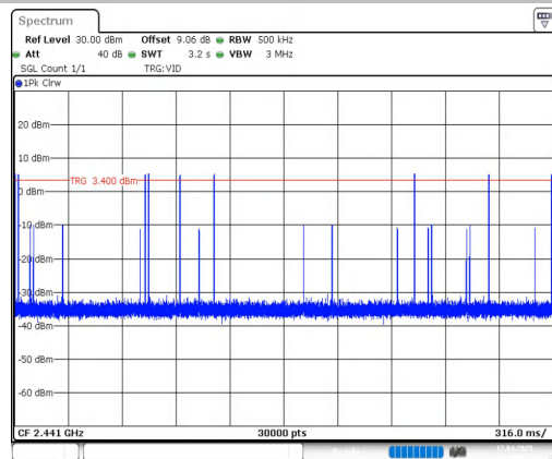
3DH3-Ant1-Hop-PASS
