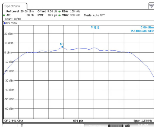
2DH5-Ant1-2441-0~Reference-PASS
