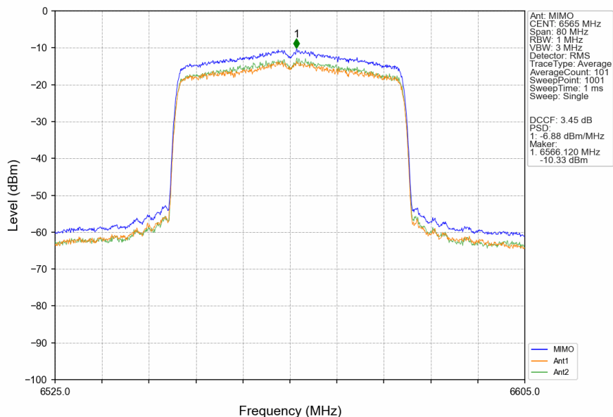
802.11ax(HEW40)_LCH_6565MHz_RU484_Left_MIMO_NTNV
