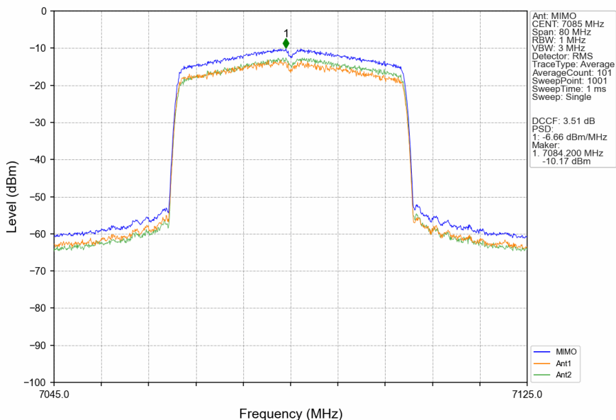
802.11ax(HEW40)_HCH_7085MHz_RU484_Left_MIMO_NTNV
