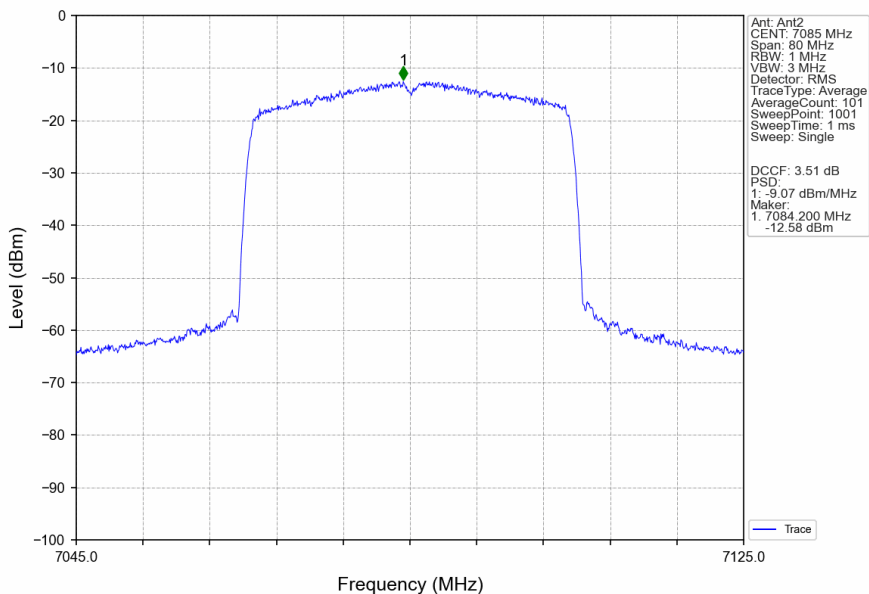
802.11ax(HEW40)_HCH_7085MHz_RU484_Left_MIMO_NTNV
