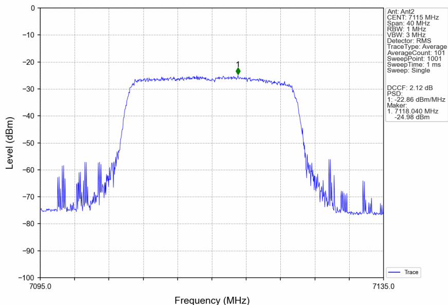
802.11ax(HEW20)_HCH_7115MHz_RU242_Left_Ant2_NTNV
