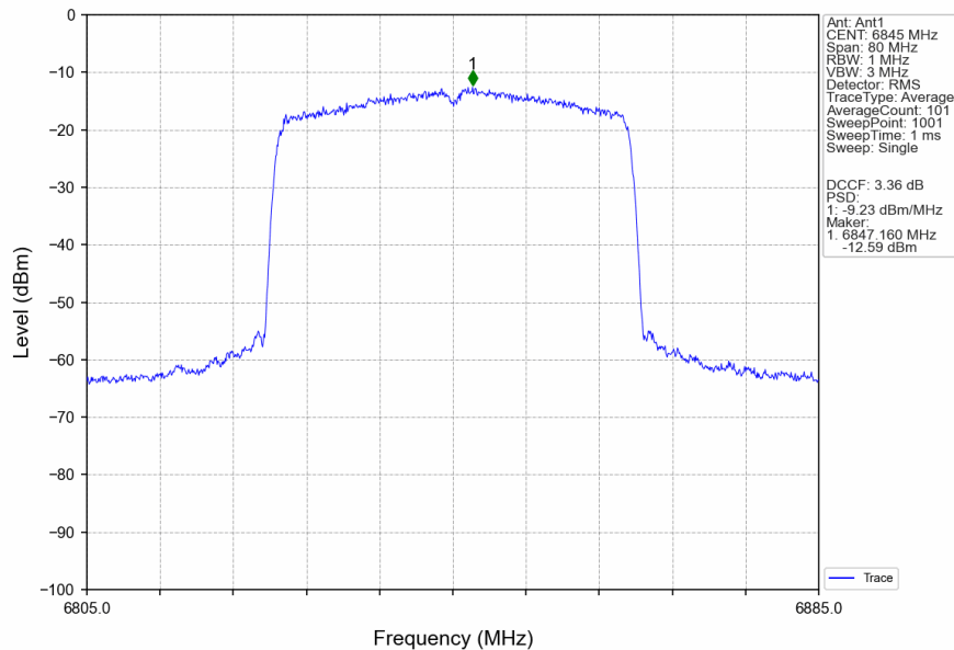
802.11ax(HEW40)_HCH_6845MHz_RU484_Left_Ant1_NTNV
