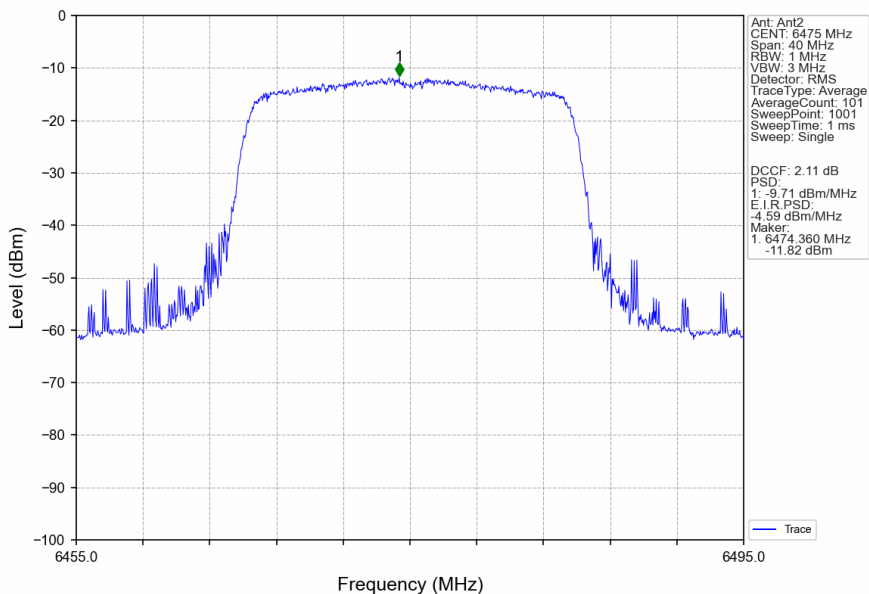
802.11ax(HEW20)_MCH_6475MHz_RU242_Left_MIMO_NTNV
