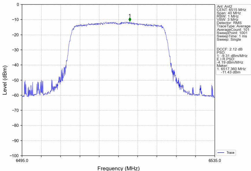
802.11ax(HEW20)_HCH_6515MHz_RU242_Left_Ant2_NTNV
