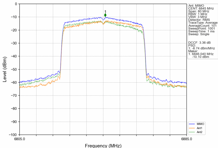
802.11ax(HEW40)_HCH_6845MHz_RU484_Left_MIMO_NTNV
