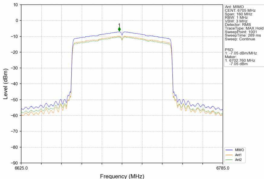
802.11ax(HEW80)_MCH_6705MHz_RU996_Left_MIMO_NTNV
