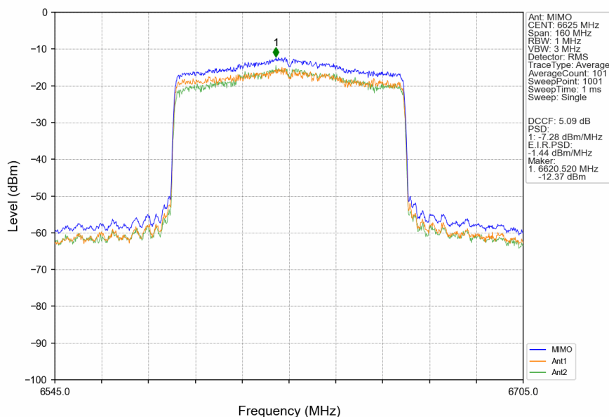
802.11ax(HEW80)_LCH_6625MHz_RU996_Left_MIMO_NTNV
