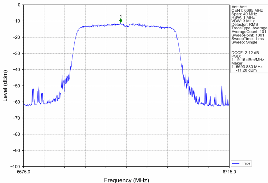
802.11ax(HEW20)_MCH_6695MHz_RU242_Left_Ant1_NTNV
