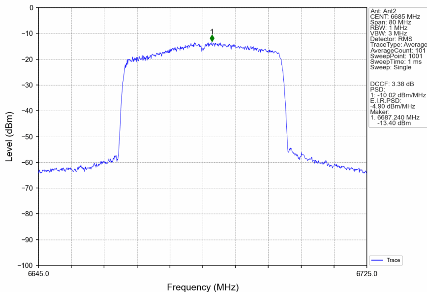
802.11ax(HEW40)_MCH_6685MHz_RU484_Left_MIMO_NTNV
