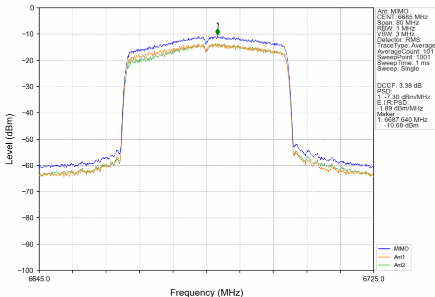
802.11ax(HEW40)_MCH_6685MHz_RU484_Left_MIMO_NTNV
