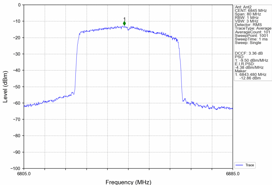
802.11ax(HEW40)_HCH_6845MHz_RU484_Left_Ant2_NTNV
