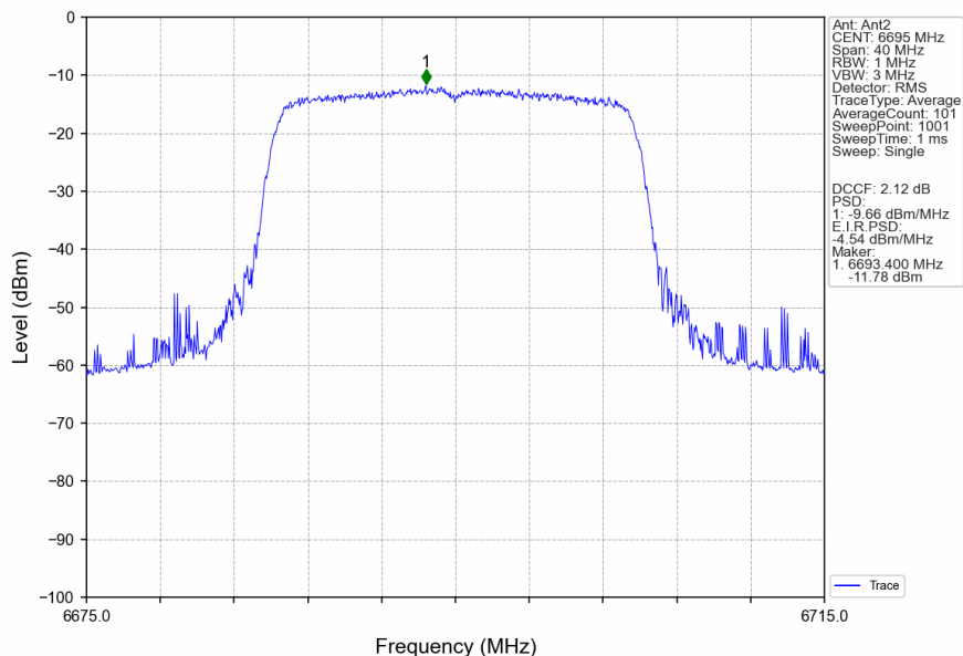
802.11ax(HEW20)_MCH_6695MHz_RU242_Left_Ant2_NTNV
