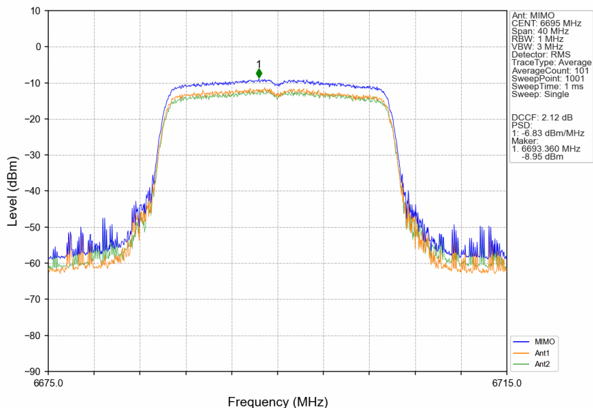
802.11ax(HEW20)_MCH_6695MHz_RU242_Left_MIMO_NTNV
