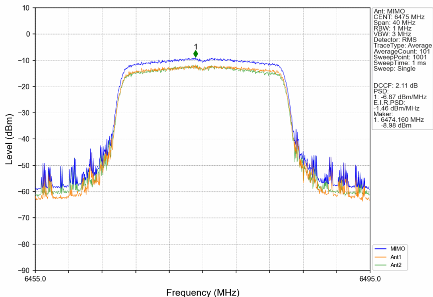
802.11ax(HEW20)_MCH_6475MHz_RU242_Left_MIMO_NTNV
