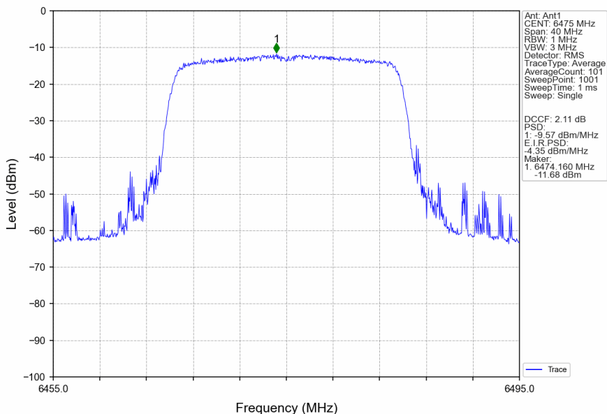
802.11ax(HEW20)_MCH_6475MHz_RU242_Left_Ant1_NTNV
