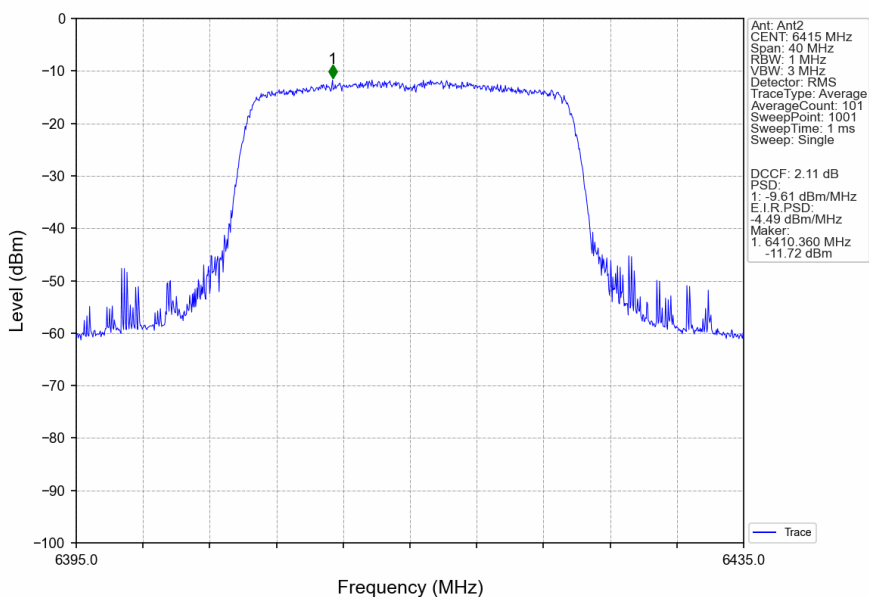
802.11ax(HEW20)_HCH_6415MHz_RU242_Left_Ant2_NTNV
