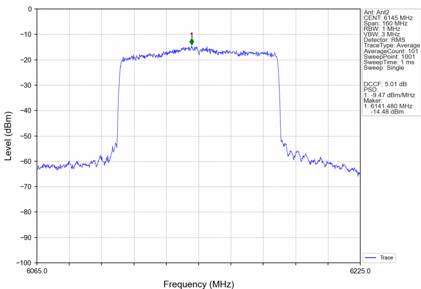
802.11ax(HEW80)_MCH_6145MHz_RU996_Left_Ant2_NTNV
