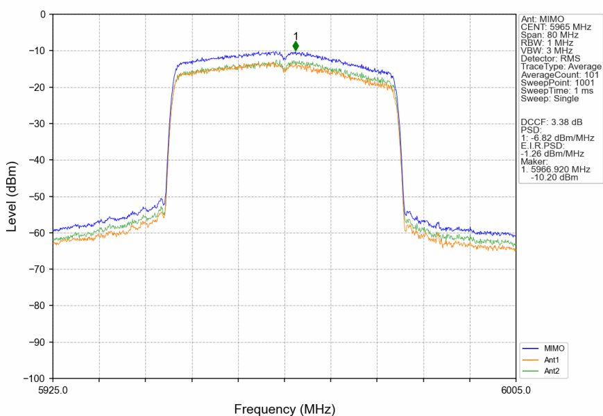
802.11ax(HEW40)_LCH_5965MHz_RU484_Left_MIMO_NTNV
