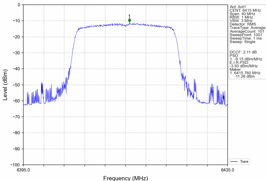
802.11ax(HEW20)_HCH_6415MHz_RU242_Left_Ant1_NTNV
