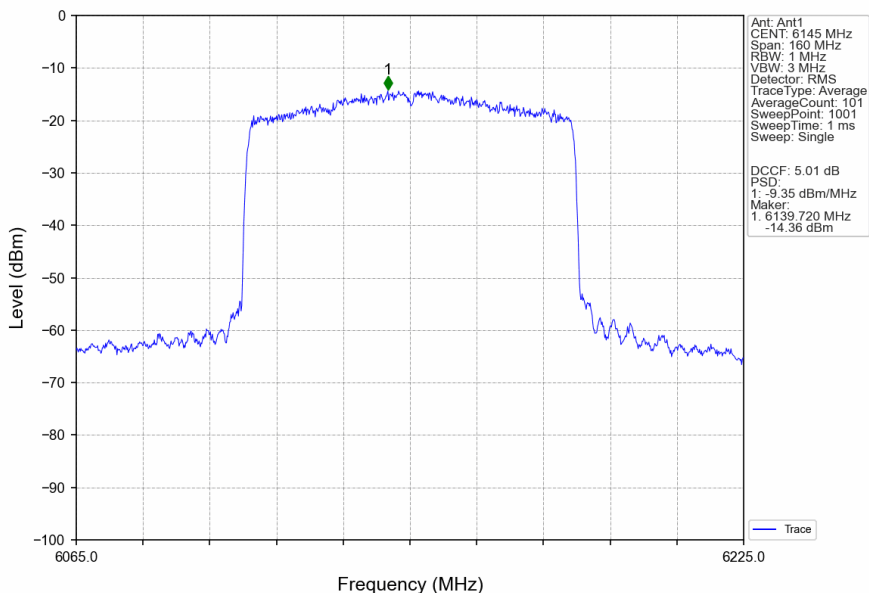
802.11ax(HEW80)_MCH_6145MHz_RU996_Left_Ant1_NTNV
