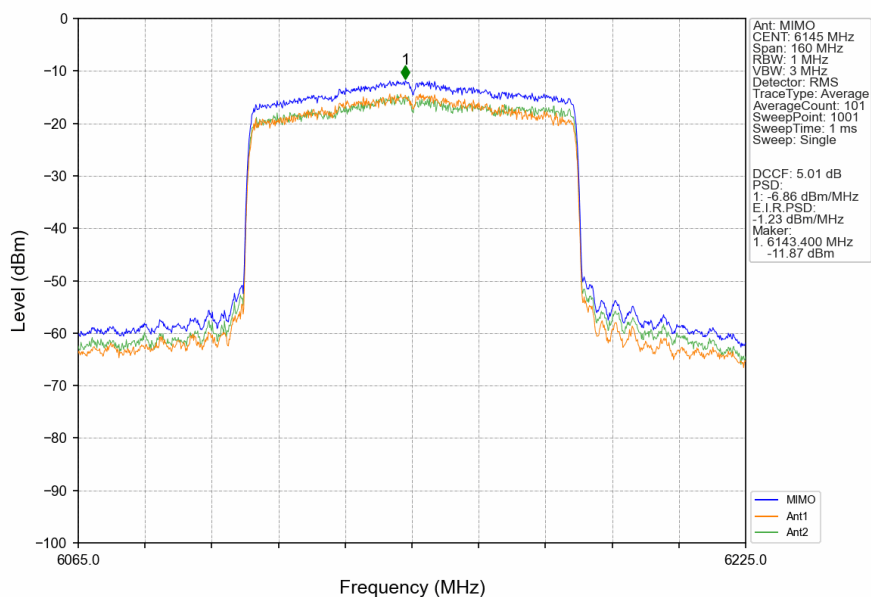
802.11ax(HEW80)_MCH_6145MHz_RU996_Left_MIMO_NTNV
