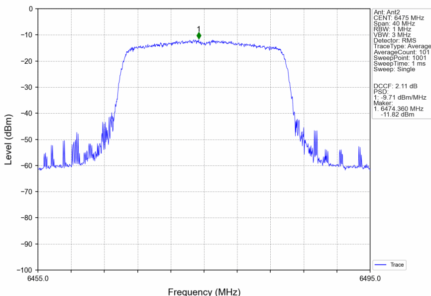
802.11ax(HEW20)_MCH_6475MHz_RU242_Left_Ant2_NTNV
