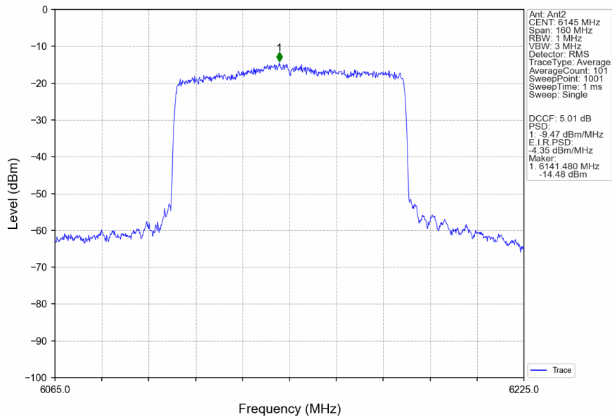
802.11ax(HEW80)_MCH_6145MHz_RU996_Left_Ant2_NTNV
