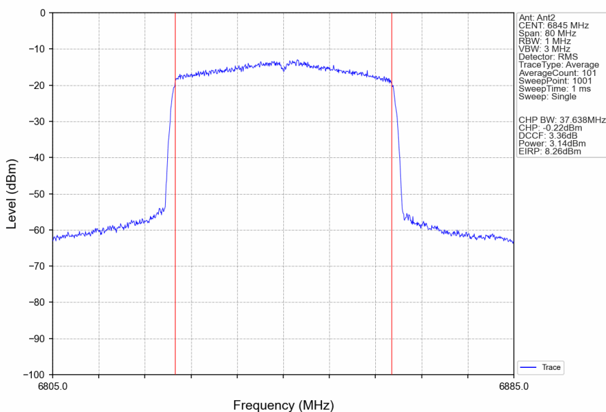
802.11ax(HEW40)_HCH_6845MHz_RU484_Left_Ant2_NTNV
