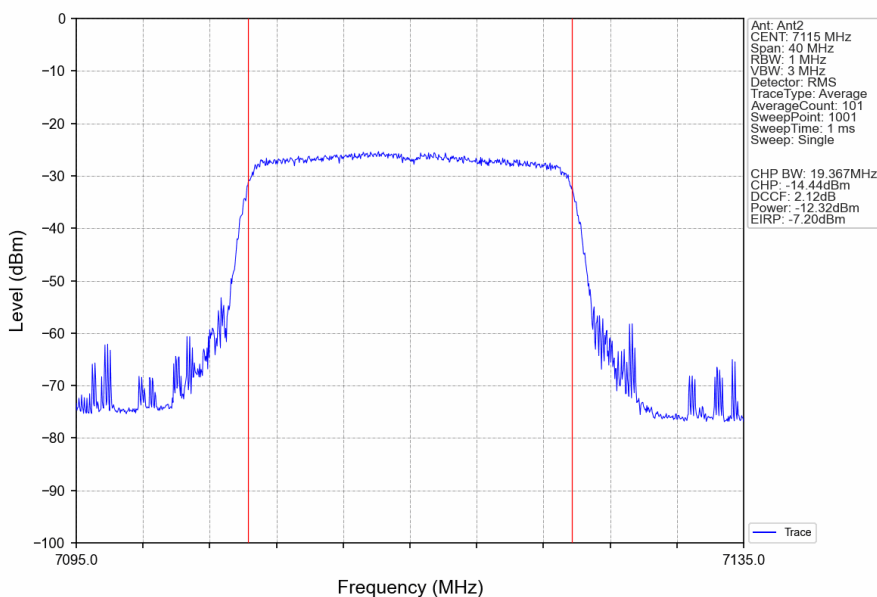
802.11ax(HEW20)_HCH_7115MHz_RU242_Left_Ant2_NTNV
