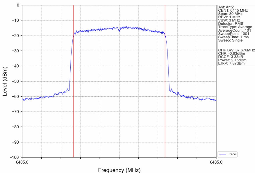
802.11ax(HEW40)_LCH_6445MHz_RU484_Left_Ant2_NTNV
