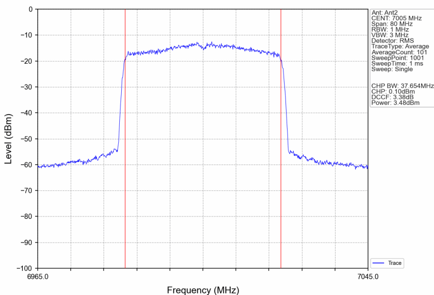
802.11ax(HEW40)_MCH_7005MHz_RU484_Left_Ant2_NTNV
