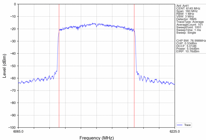
802.11ax(HEW80)_MCH_6145MHz_RU996_Left_Ant1_NTNV
