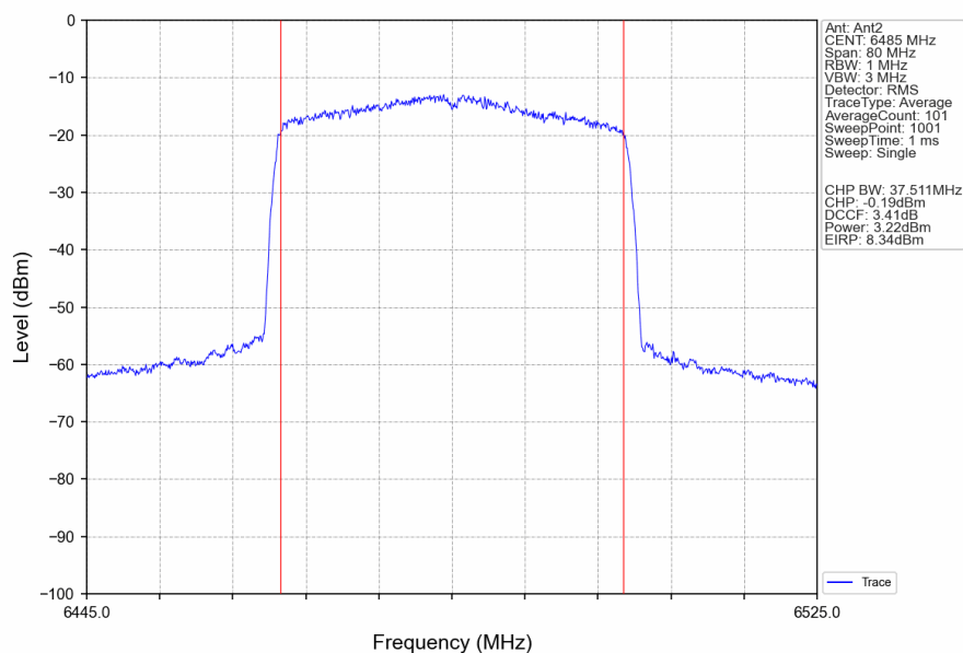
802.11ax(HEW40)_MCH_6485MHz_RU484_Left_Ant2_NTNV
