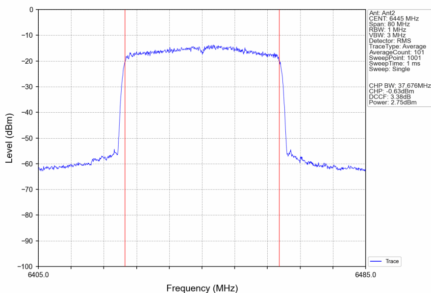
802.11ax(HEW40)_LCH_6445MHz_RU484_Left_Ant2_NTNV
