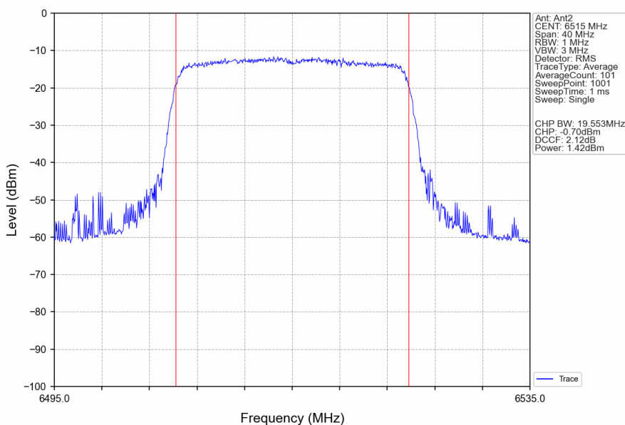
802.11ax(HEW20)_HCH_6515MHz_RU242_Left_Ant2_NTNV
