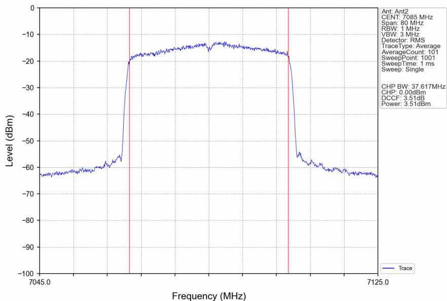
802.11ax(HEW40)_HCH_7085MHz_RU484_Left_Ant2_NTNV
