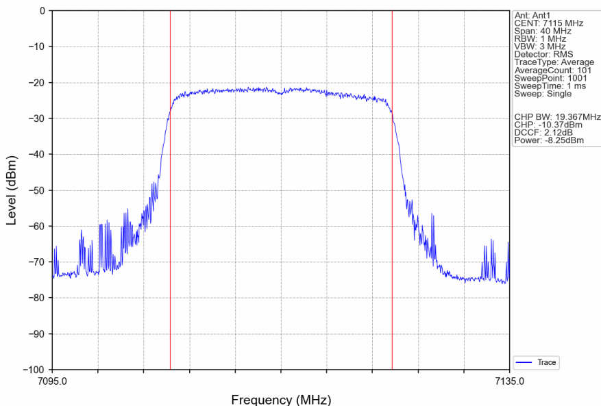
802.11ax(HEW20)_HCH_7115MHz_RU242_Left_Ant1_NTNV
