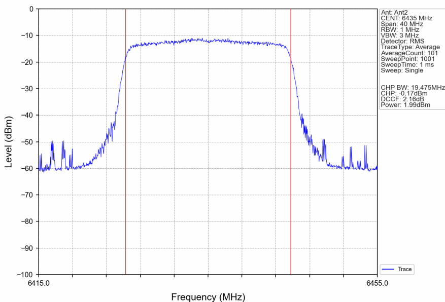
802.11ax(HEW20)_LCH_6435MHz_RU242_Left_Ant2_NTNV
