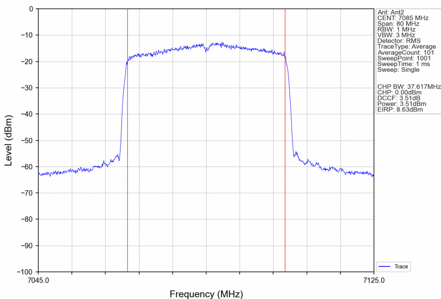
802.11ax(HEW40)_HCH_7085MHz_RU484_Left_Ant2_NTNV
