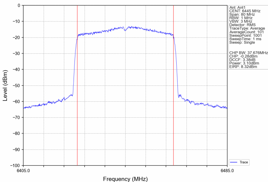
802.11ax(HEW40)_LCH_6445MHz_RU484_Left_Ant1_NTNV
