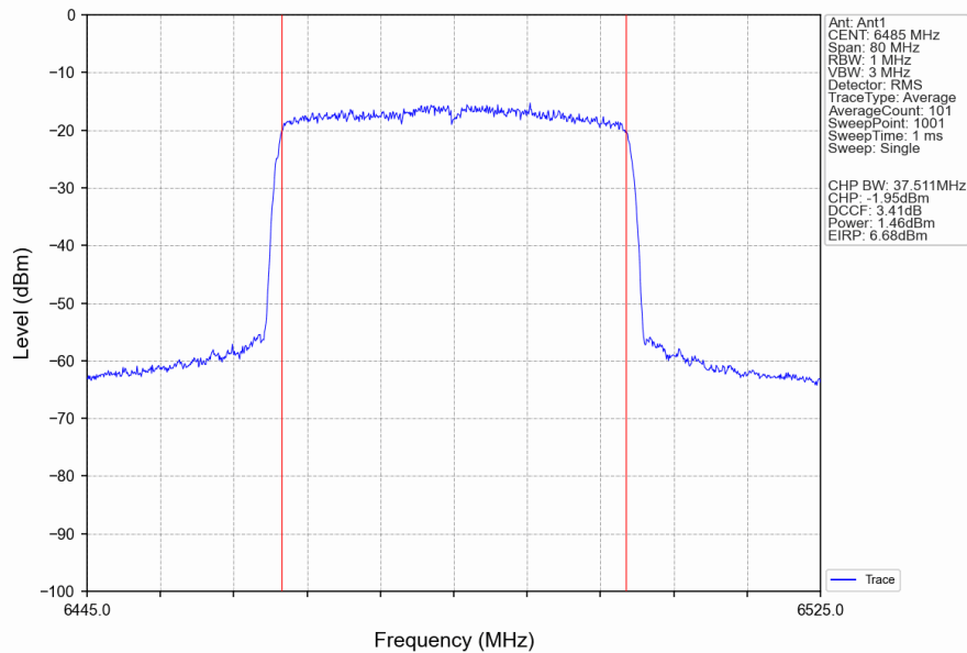
802.11ax(HEW40)_MCH_6485MHz_RU484_Left_Ant1_NTNV
