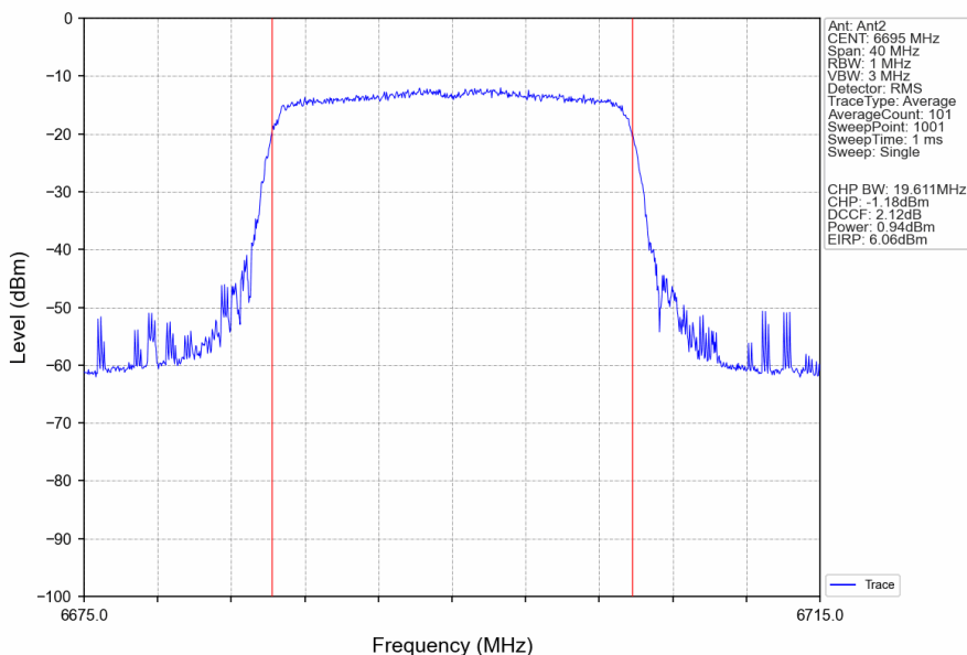
802.11ax(HEW20)_MCH_6695MHz_RU242_Left_Ant2_NTNV
