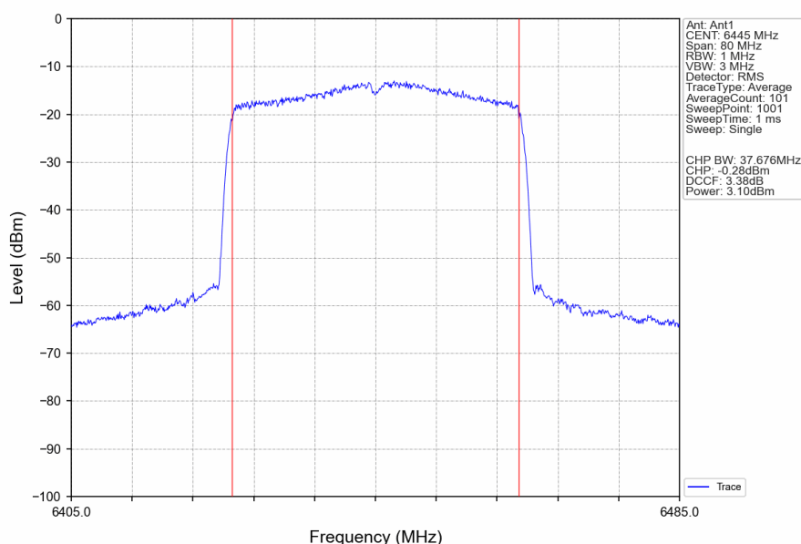
802.11ax(HEW40)_LCH_6445MHz_RU484_Left_Ant1_NTNV
