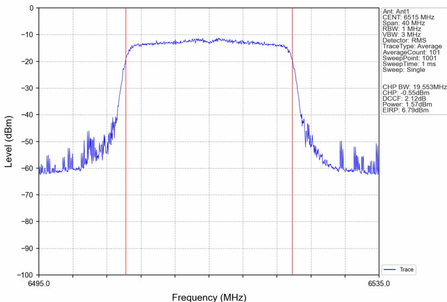
802.11ax(HEW20)_HCH_6515MHz_RU242_Left_Ant1_NTNV
