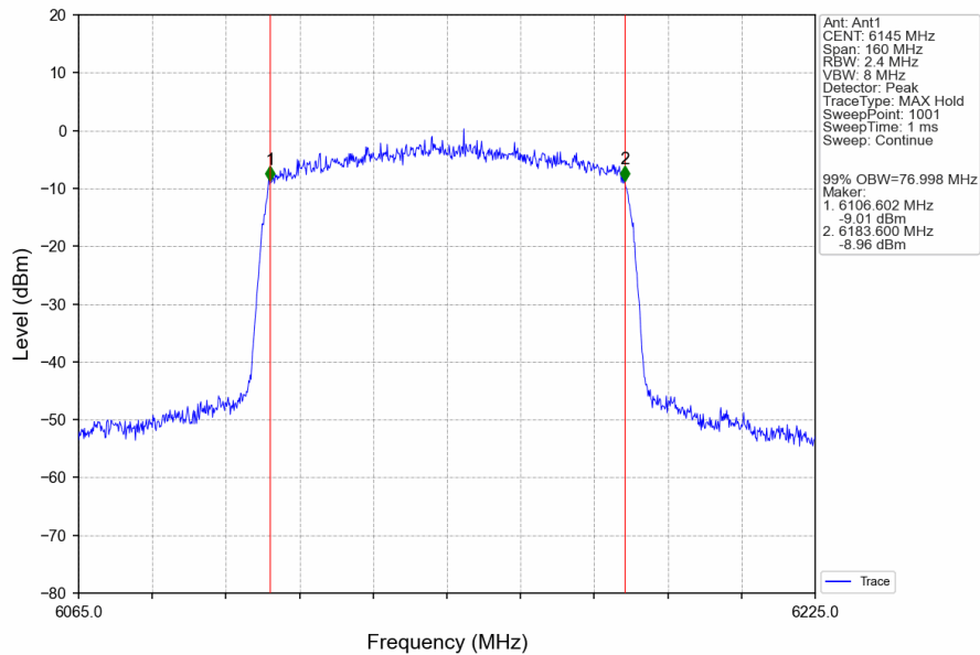
802.11ax(HEW80)_MCH_6145MHz_RU996_Left_Ant1_NTNV
