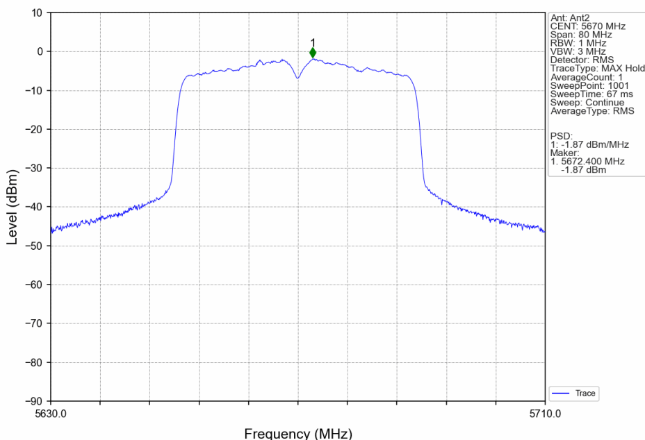
802.11ax(HEW40)_HCH_5670MHz_SU_/_MIMO_NTNV
