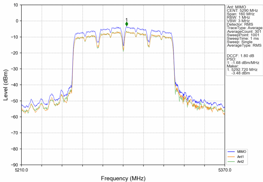
802.11ax(HEW80)_MCH_5290MHz_SU_/_MIMO_NTNV
