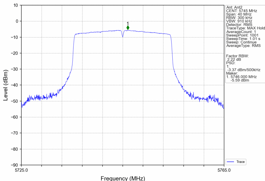
802.11ax(HEW20)_LCH_5745MHz_SU_ / _MIMO_NTNV
