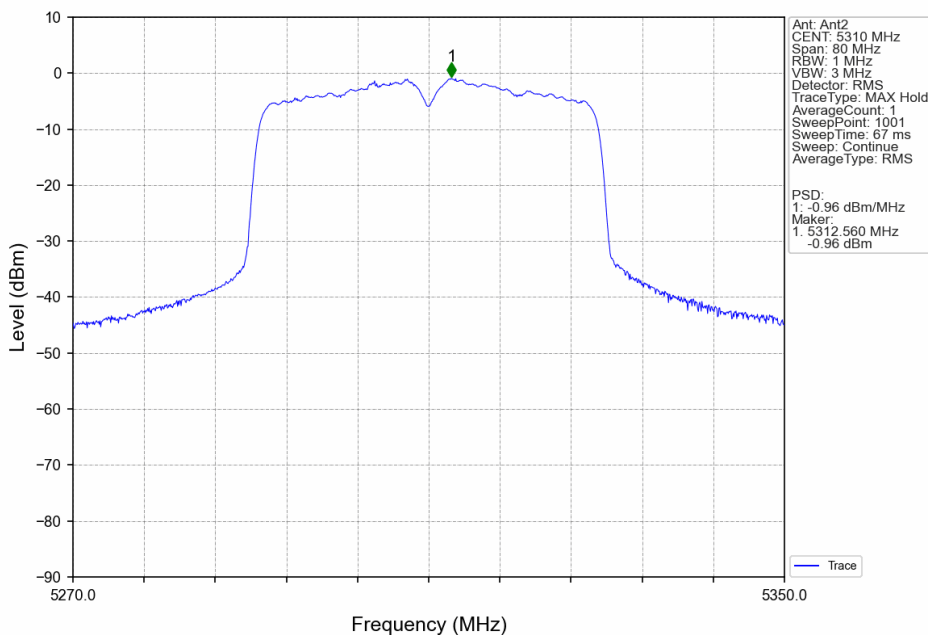
802.11ax(HEW40)_HCH_5310MHz_SU_/_Ant2_NTNV
