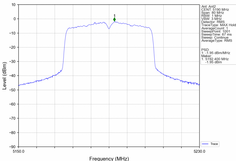
802.11ax(HEW40)_LCH_5190MHz_SU_ / _MIMO_NTNV
