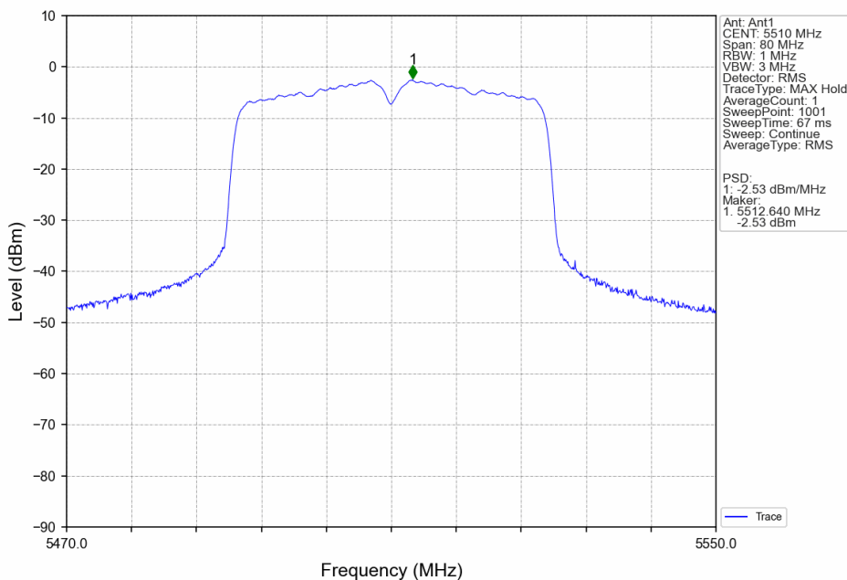
802.11ax(HEW40)_LCH_5510MHz_SU_/_Ant1_NTNV
