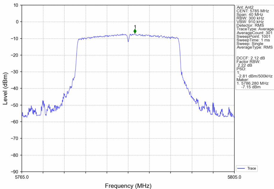
802.11ax(HEW20)_MCH_5785MHz_SU_ / _Ant2_NTNV
