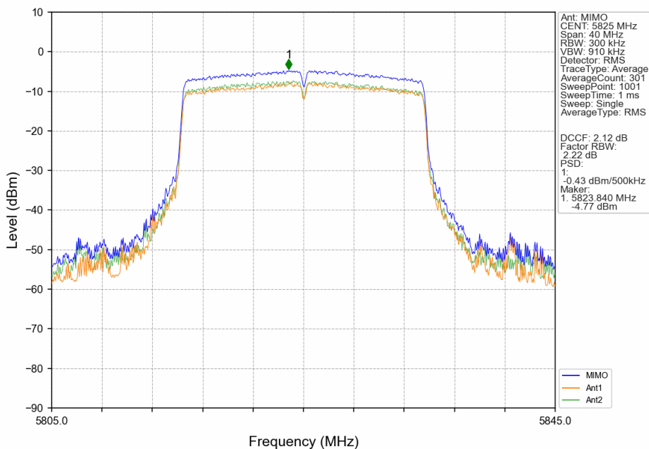
802.11ax(HEW20)_HCH_5825MHz_SU_/_MIMO_NTNV
