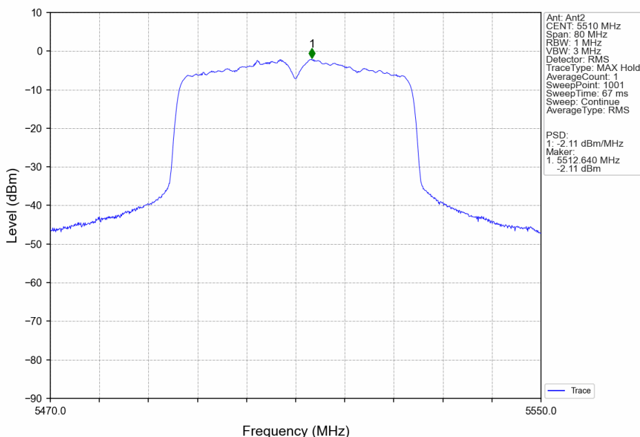
802.11ax(HEW40)_LCH_5510MHz_SU_ / _MIMO_NTNV
