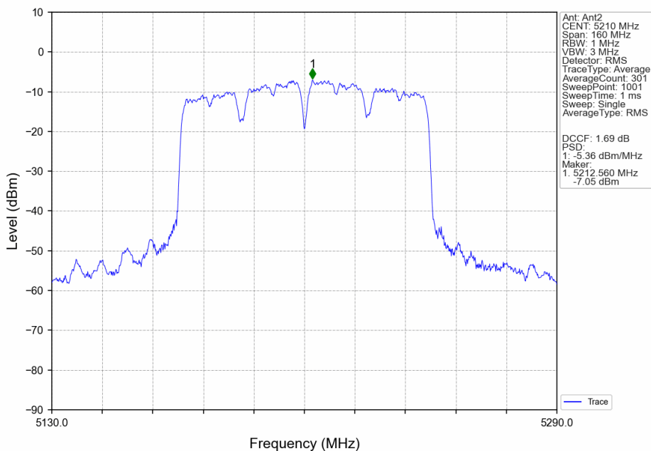
802.11ax(HEW80)_MCH_5210MHz_SU_/_Ant2_NTNV
