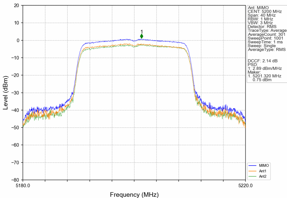
802.11ax(HEW20)_MCH_5200MHz_SU_/_MIMO_NTNV
