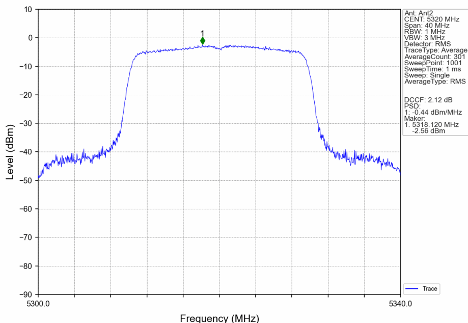
802.11ax(HEW20)_HCH_5320MHz_SU_/_MIMO_NTNV
