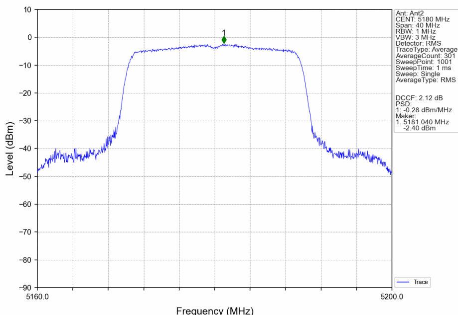
802.11ax(HEW20)_LCH_5180MHz_SU_ / _Ant2_NTNV
