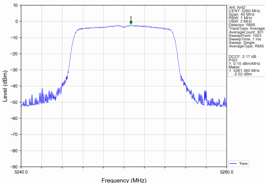
802.11ax(HEW20)_LCH_5260MHz_SU_/_MIMO_NTNV
