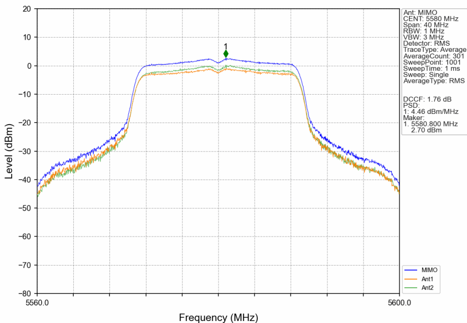
802.11ac(VHT20)_MCH_5580MHz_MIMO_NTNV
