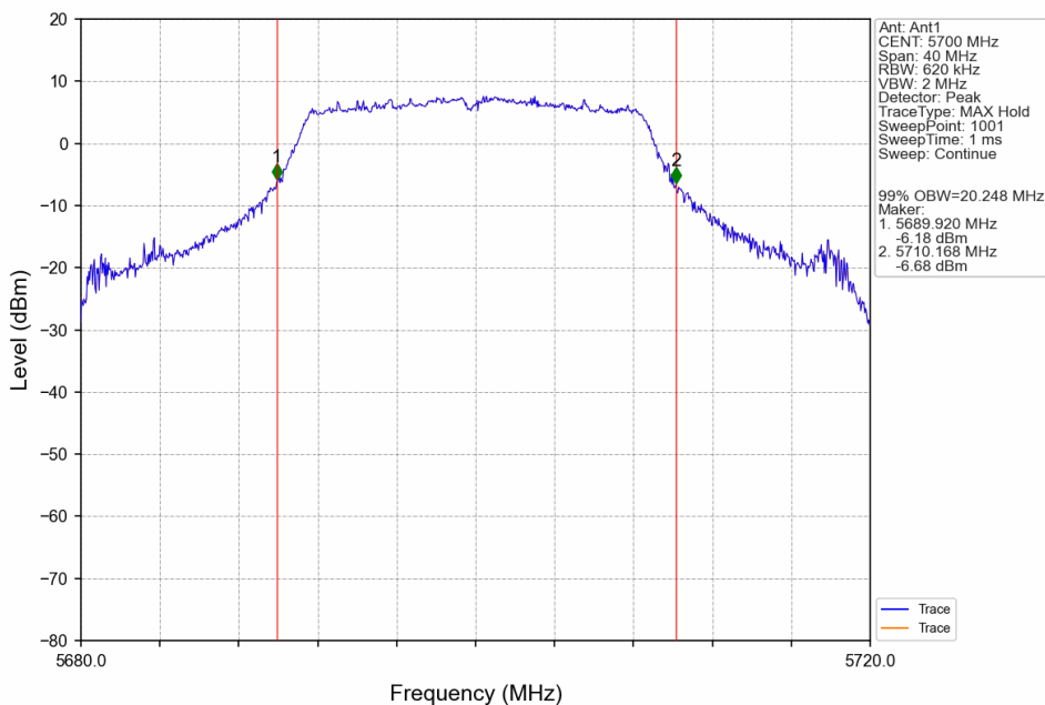
802.11ax(HEW20)_HCH_5700MHz_SU_/_Ant1_NTNV
