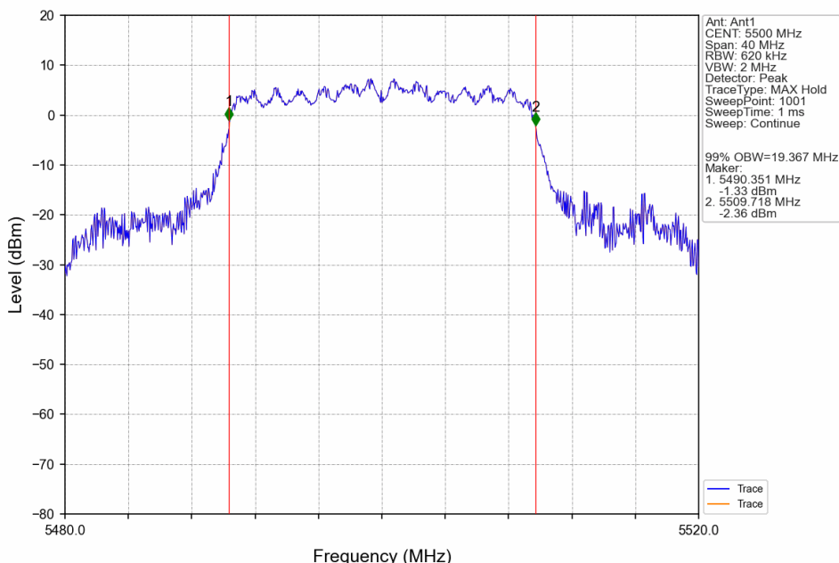
802.11ax(HEW20)_LCH_5500MHz_SU_/_Ant1_NTNV
