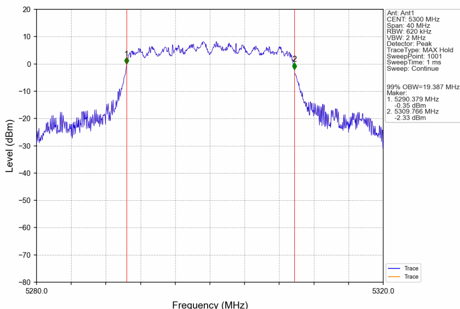
802.11ax(HEW20)_MCH_5300MHz_SU_/_Ant1_NTNV
