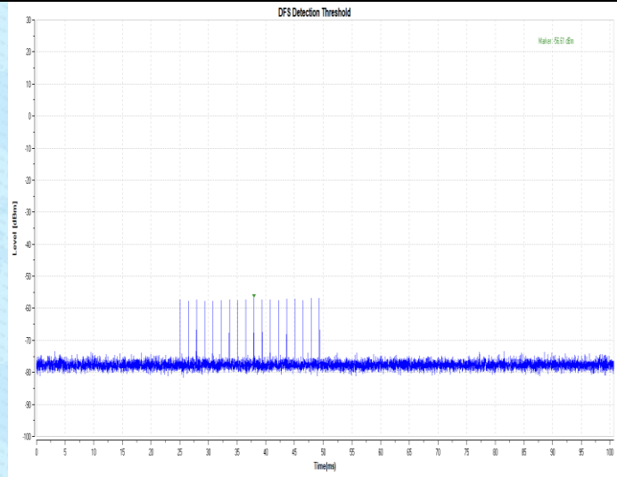
11N40SISO-5510-Type0-PASS
