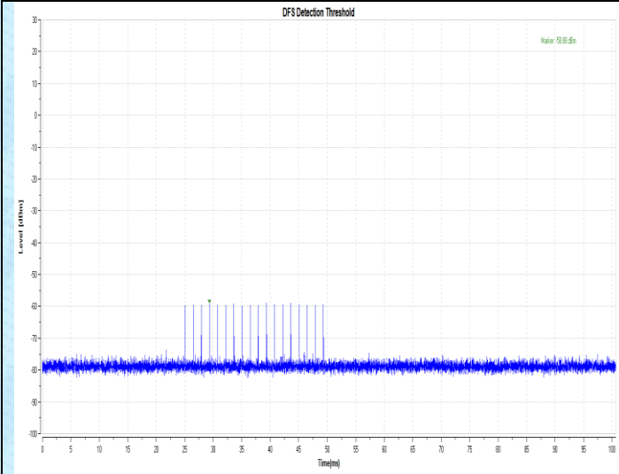
11N40SISO-5270-Type0-PASS
