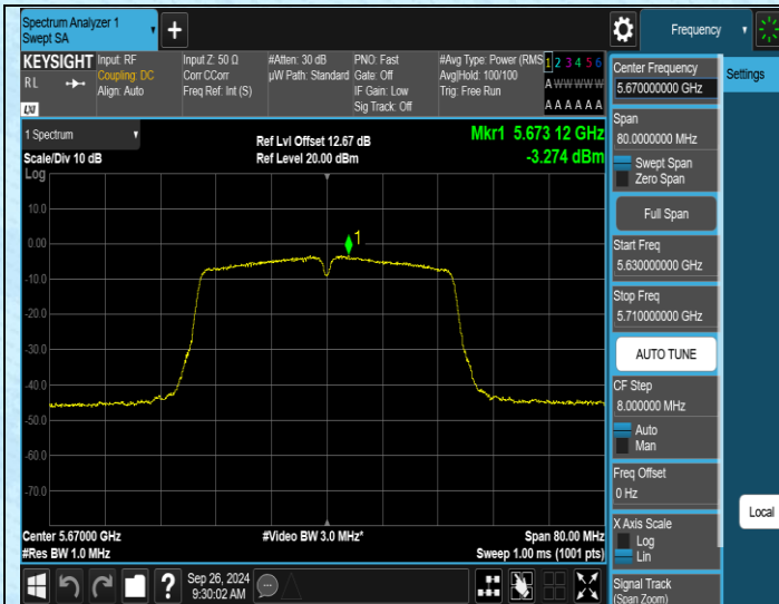
11AC40SISO-Ant1-5670-PASS
