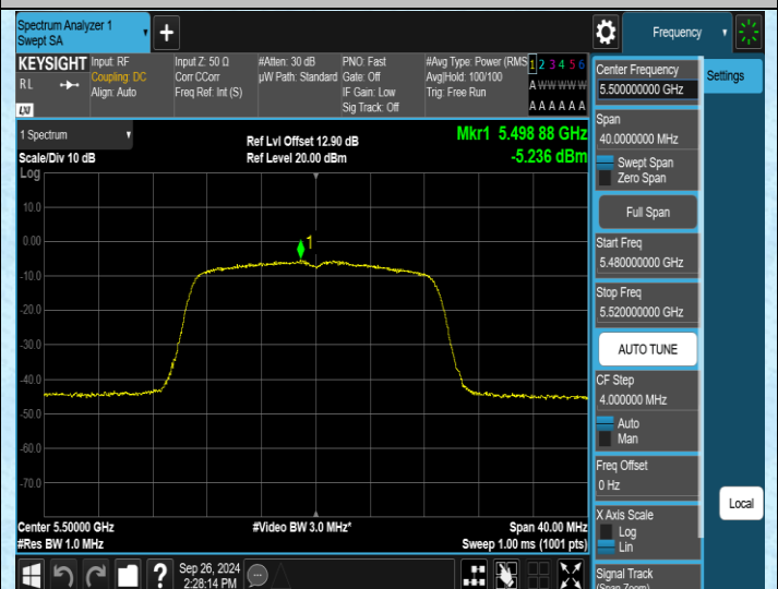
11N20MIMO-Ant2-5500-PASS
