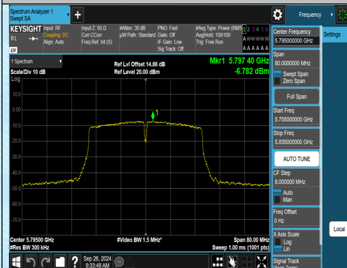
11AC40SISO-Ant1-5795-PASS
