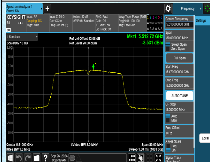
11AC40SISO-Ant1-5510-PASS
