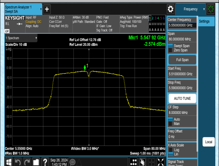
11AC40SISO-Ant2-5550-PASS
