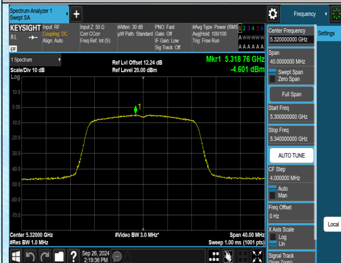
11N20MIMO-Ant1-5320-PASS
