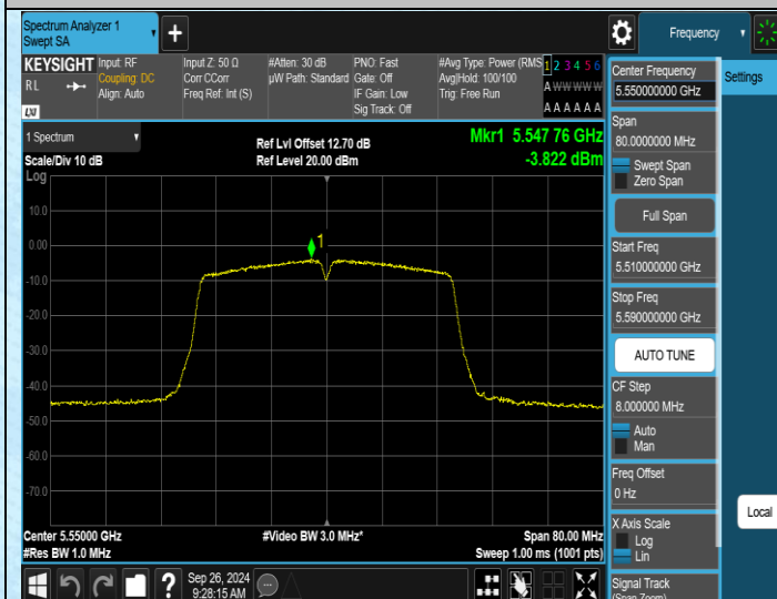
11AC40SISO-Ant1-5550-PASS
