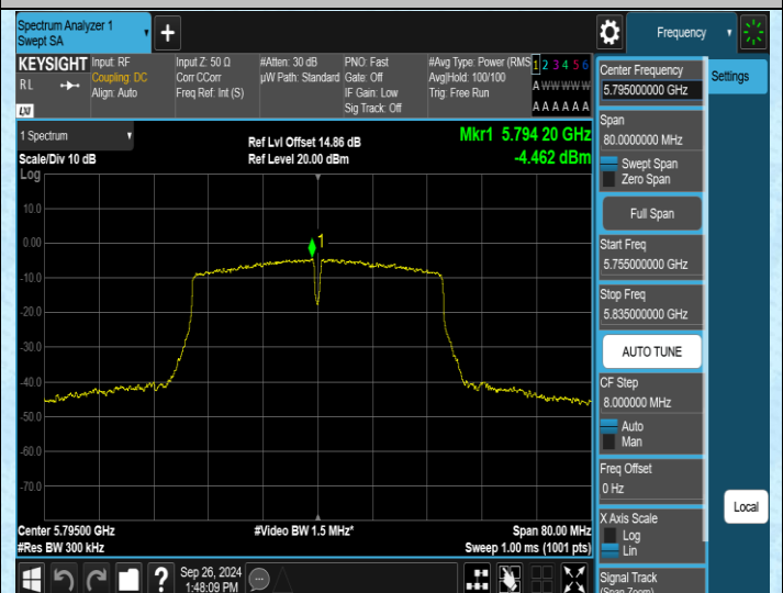
11AC40SISO-Ant2-5795-PASS
