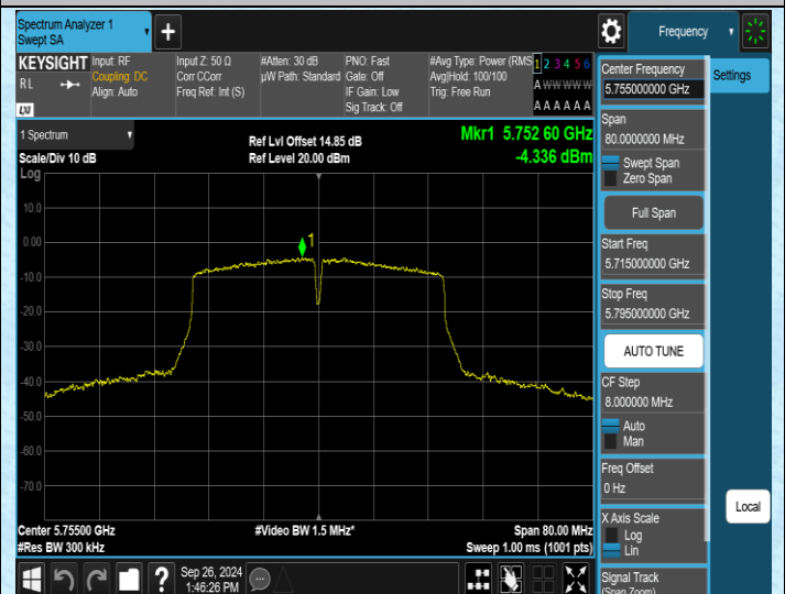
11AC40SISO-Ant2-5755-PASS
