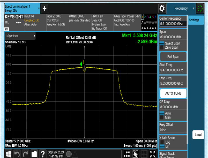
11AC40SISO-Ant2-5510-PASS
