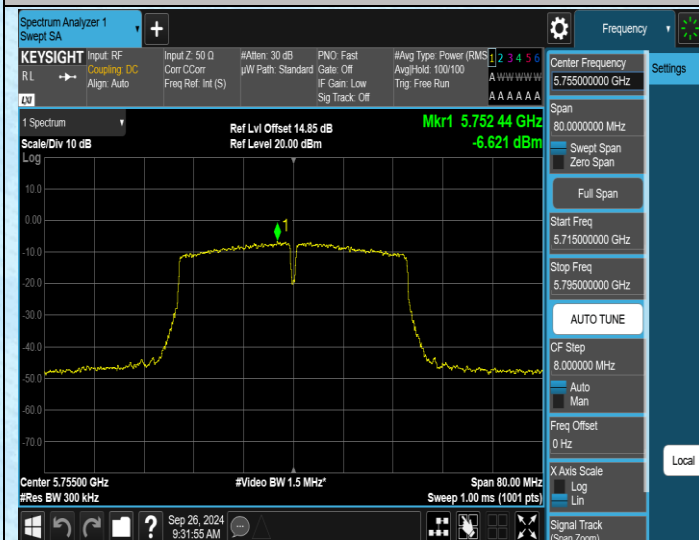
11AC40SISO-Ant1-5755-PASS
