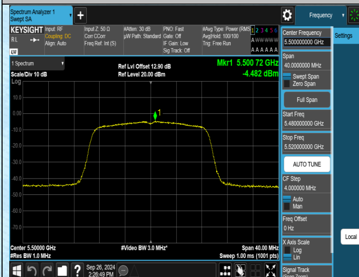
11N20MIMO-Ant1-5500-PASS
