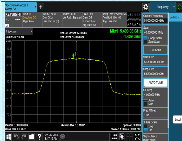
11N20SISO-Ant1-5500-PASS
