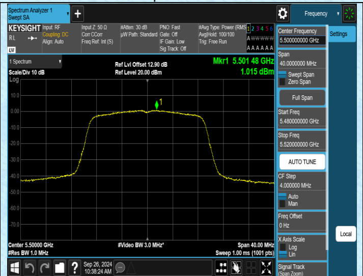
11N20SISO-Ant2-5500-PASS
