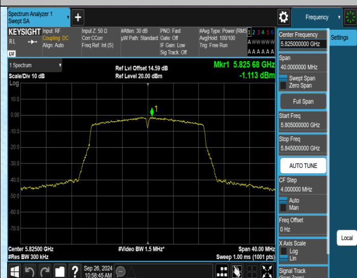
11N20SISO-Ant2-5825-PASS
