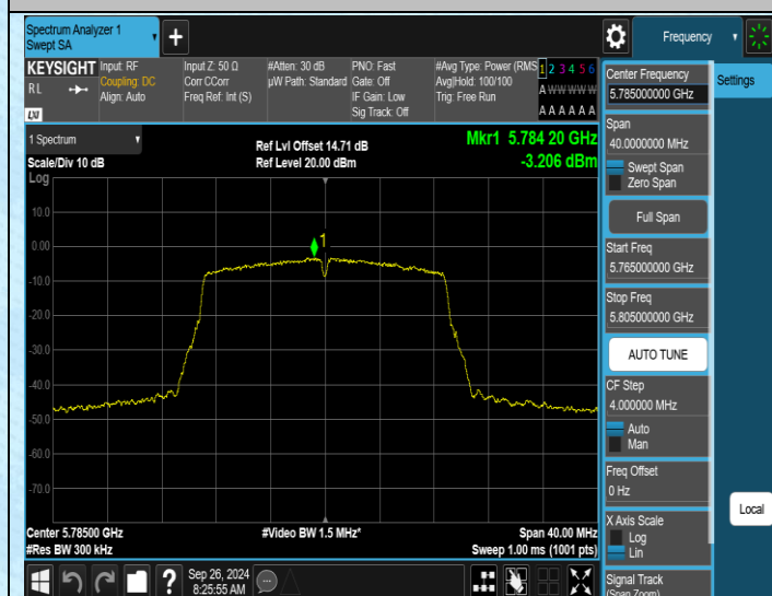
11N20SISO-Ant1-5785-PASS
