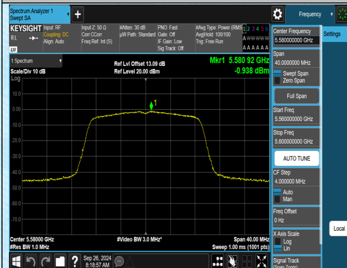
11N20SISO-Ant1-5580-PASS
