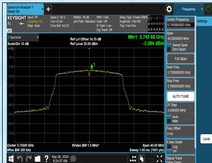
11N20SISO-Ant1-5745-PASS
