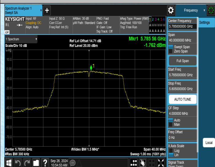
11N20SISO-Ant2-5785-PASS
