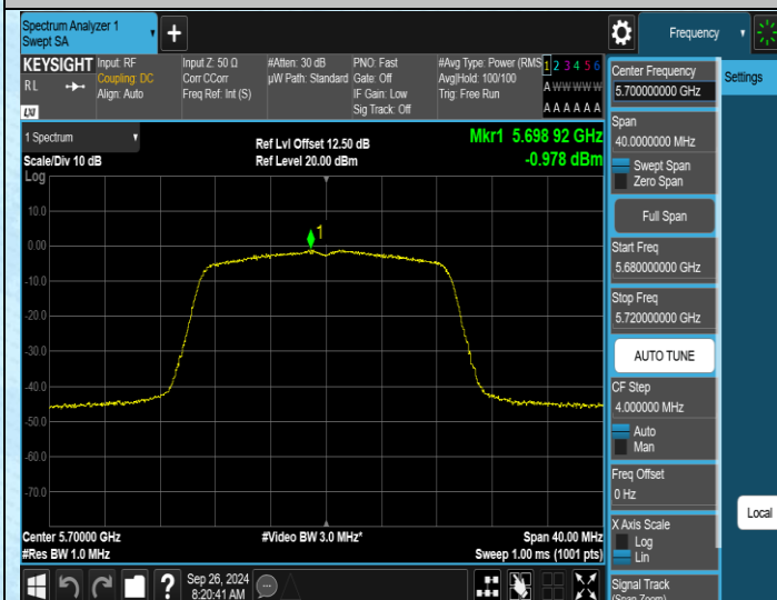
11N20SISO-Ant1-5700-PASS
