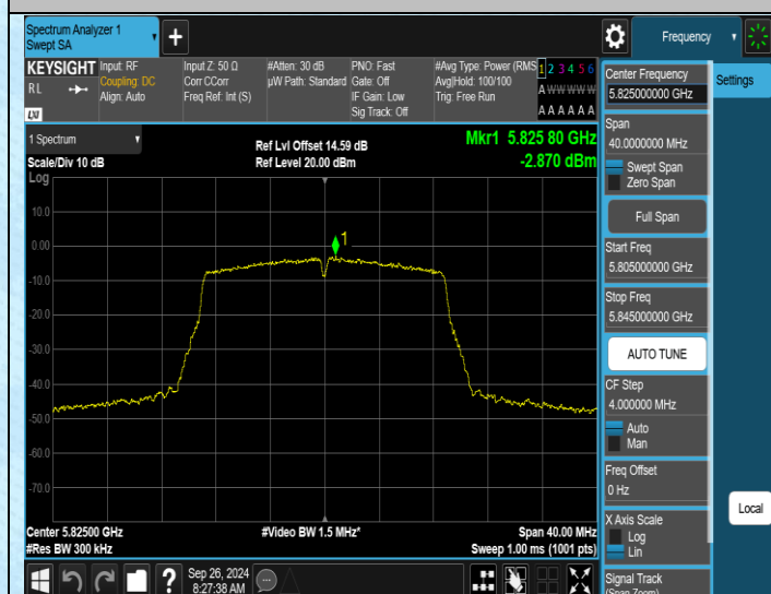
11N20SISO-Ant1-5825-PASS
