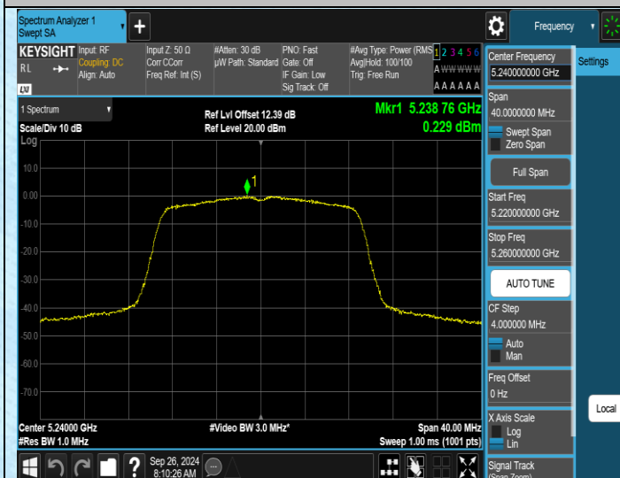
11N20SISO-Ant1-5240-PASS
