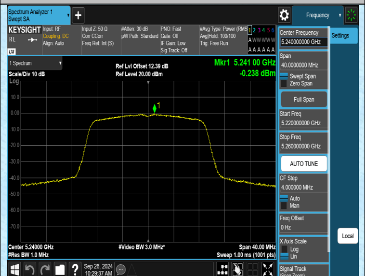
11N20SISO-Ant2-5240-PASS
