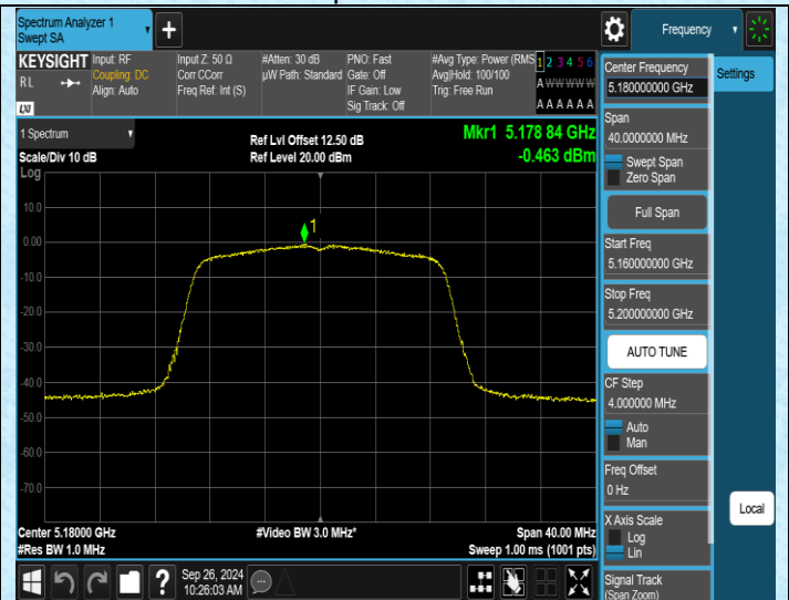
11N20SISO-Ant2-5180-PASS
