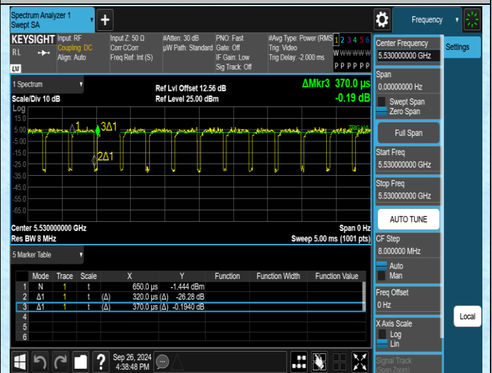
NTNV-11AC80MIMO-Ant2-5530
