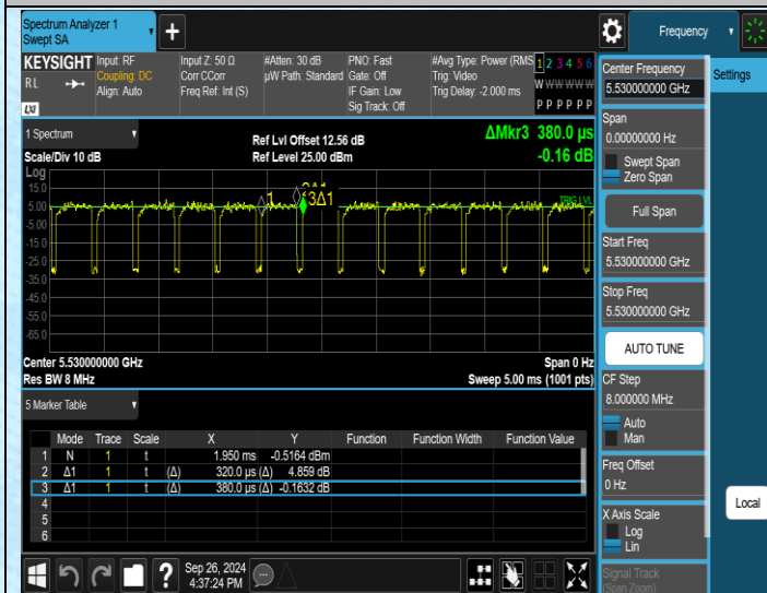
NTNV-11AC80MIMO-Ant1-5530
