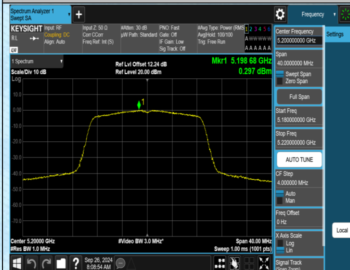
11N20SISO-Ant1-5200-PASS
