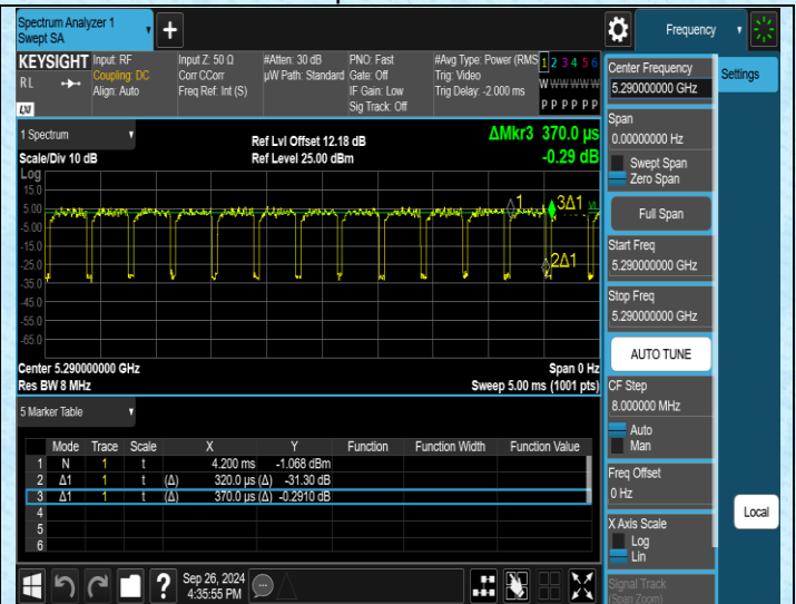
NTNV-11AC80MIMO-Ant2-5290
