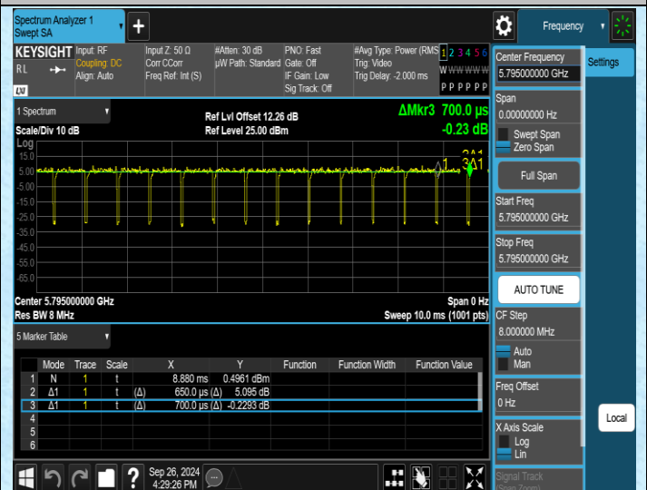
NTNV-11AC40MIMO-Ant2-5795
