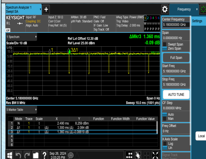
NTNV-11N20MIMO-Ant1-5180
