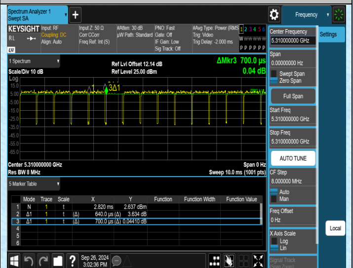
NTNV-11N40MIMO-Ant2-5310
