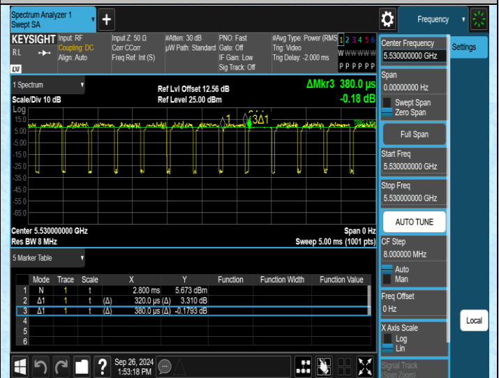
NTNV-11AC80SISO-Ant2-5530
