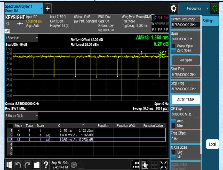
NTNV-11N20MIMO-Ant2-5785
