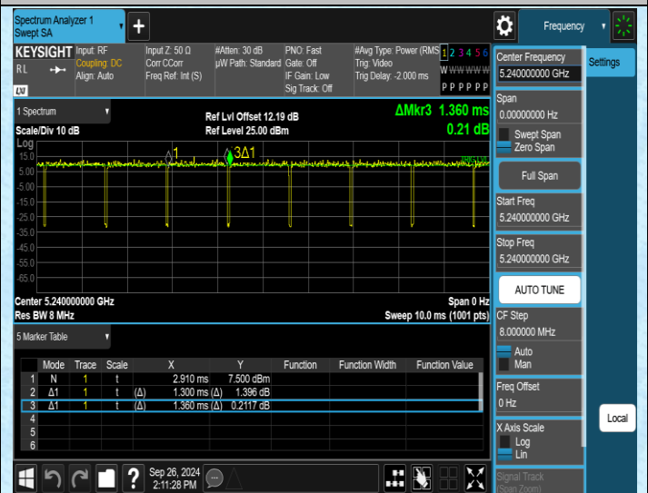
NTNV-11N20MIMO-Ant2-5240
