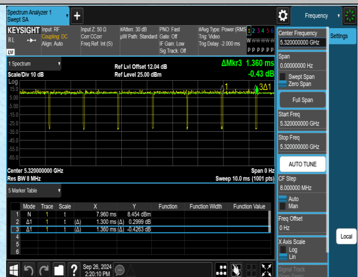
NTNV-11N20MIMO-Ant2-5320
