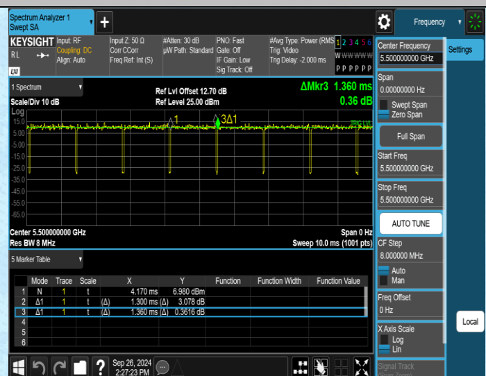
NTNV-11N20MIMO-Ant2-5500
