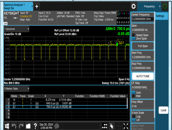
NTNV-11N40MIMO-Ant2-5230
