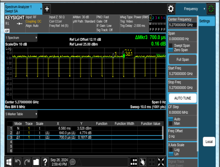
NTNV-11N40MIMO-Ant2-5270
