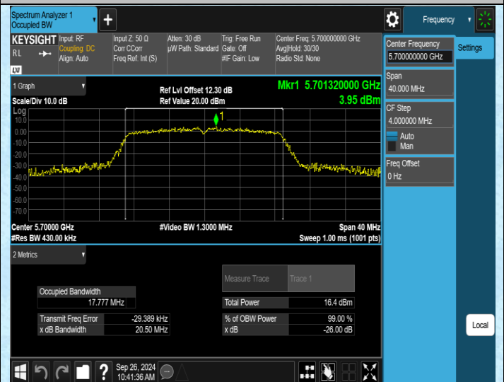
11N20SISO-Ant2-5700
