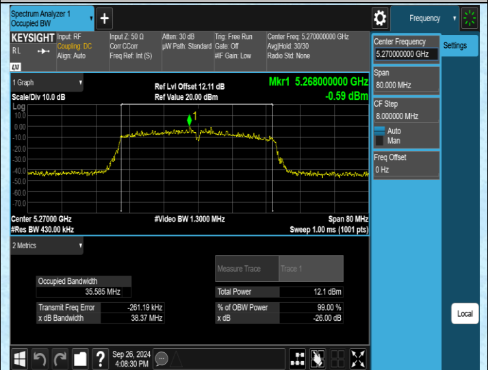
11AC40MIMO-Ant2-5270
