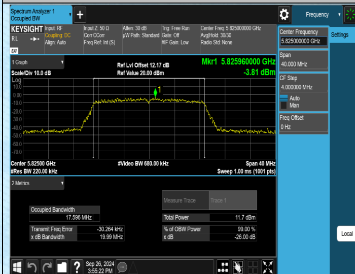
11AC20MIMO-Ant1-5825
