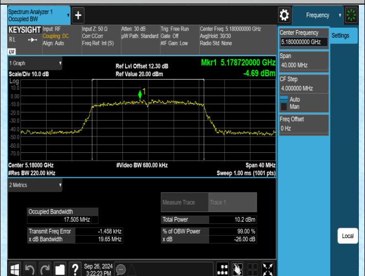
11AC20MIMO-Ant2-5180
