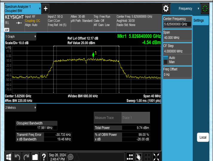
11N20MIMO-Ant2-5825
