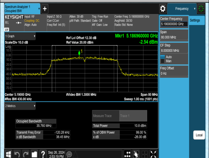
11N40MIMO-Ant2-5190
