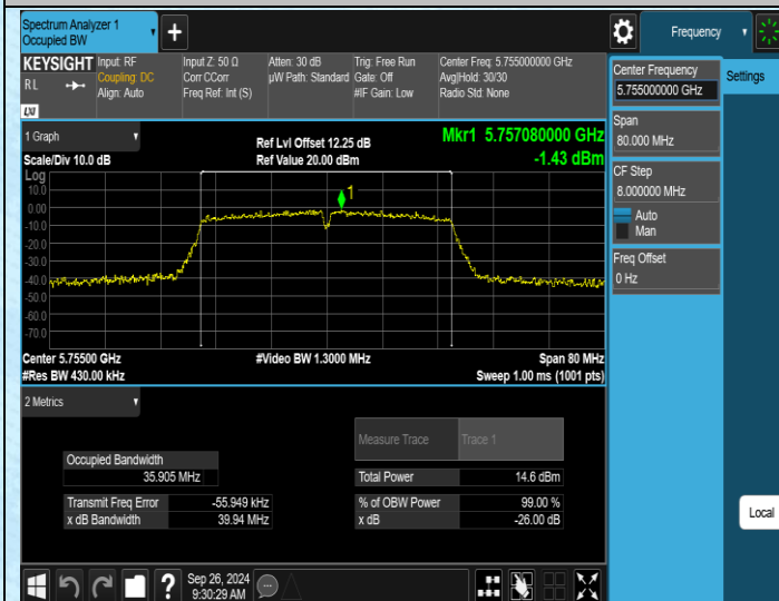
11AC40SISO-Ant1-5755
