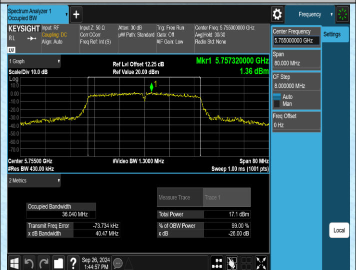
11AC40SISO-Ant2-5755
