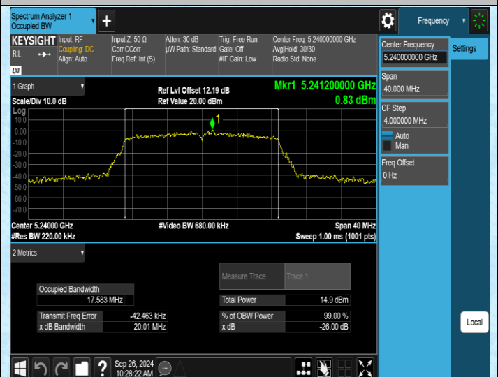
11N20SISO-Ant2-5240
