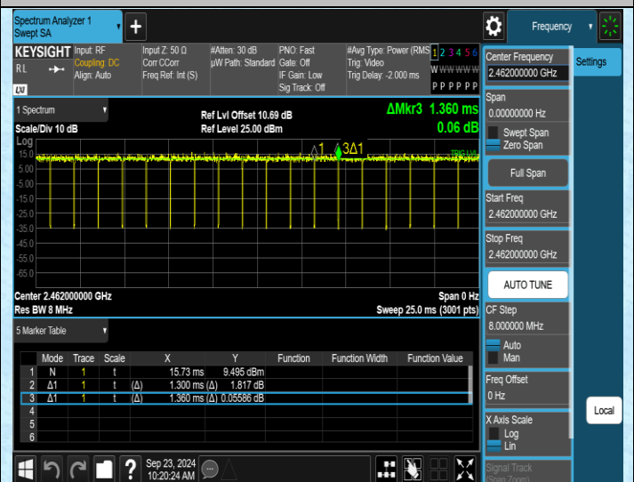
NTNV-11N20SISO-Ant2-2462
