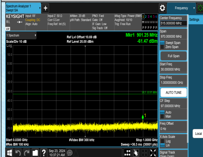
11N20MIMO-Ant2-2462-30~1000-PASS
