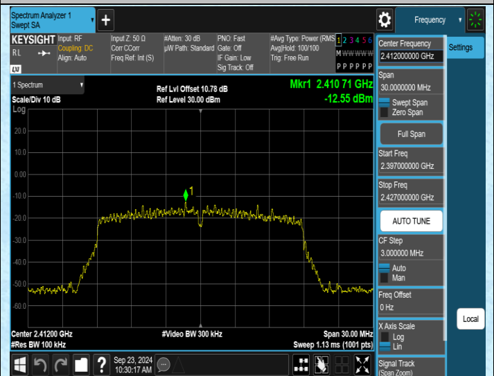
11N20MIMO-Ant2-2412-0~Reference-PASS
