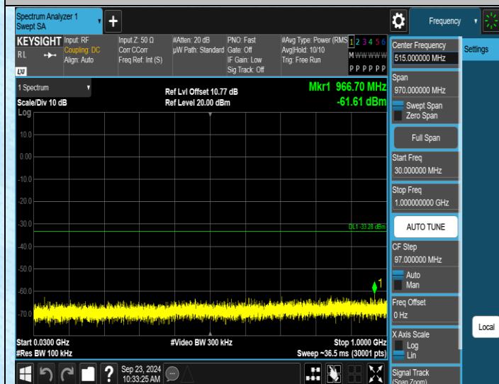
11N20MIMO-Ant2-2437-30~1000-PASS
