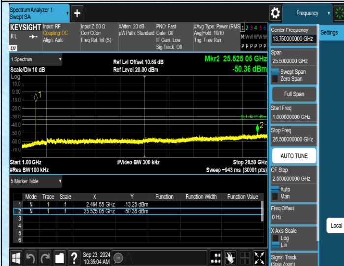
11N20MIMO-Ant1-2462-1000~26500-PASS
