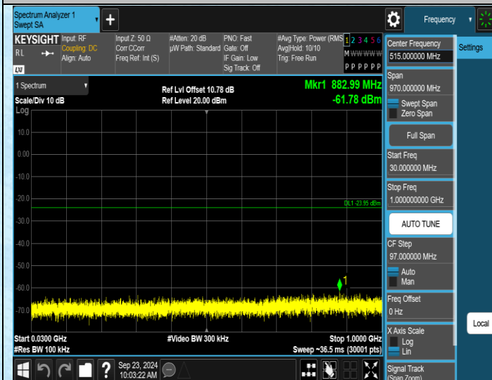
11G-Ant2-2412-30~1000-PASS
