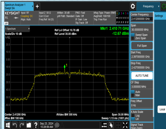
11N20MIMO-Ant1-2412-0~Reference-PASS
