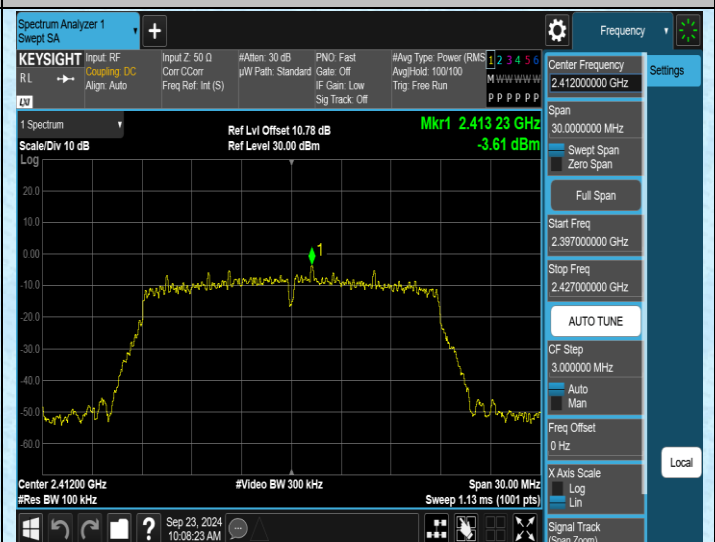
11N20SISO-Ant2-2412-0~Reference-PASS
