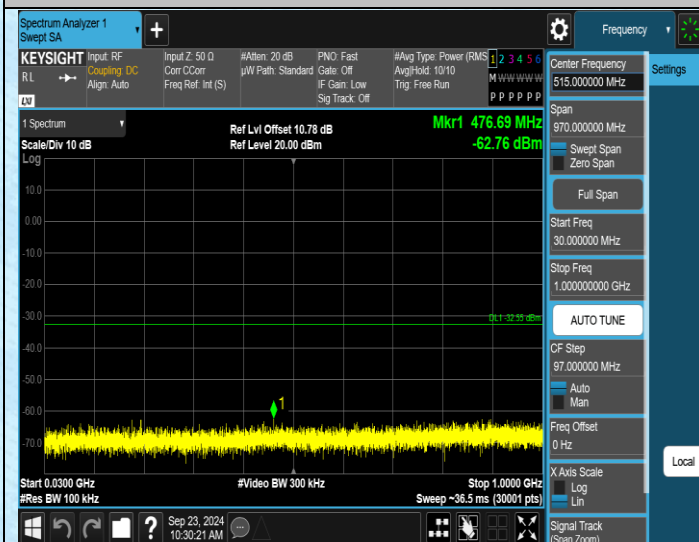
11N20MIMO-Ant2-2412-30~1000-PASS
