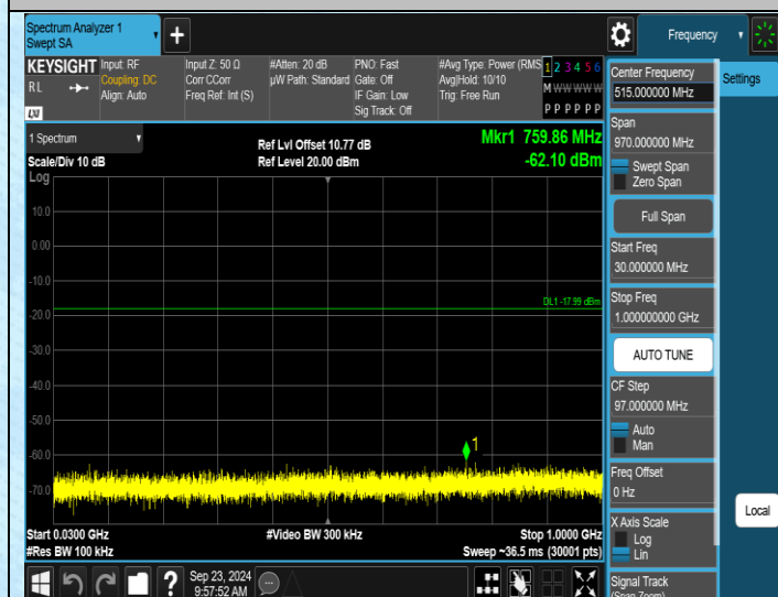
11B-Ant2-2437-30~1000-PASS
