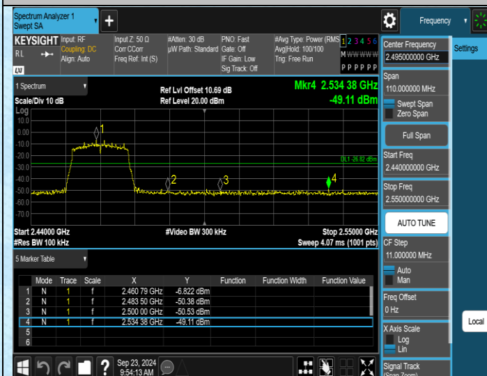
11N20SISO-Ant1-2462-PASS
