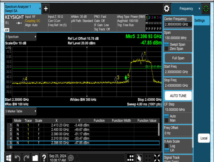
11N20SISO-Ant2-2412-PASS
