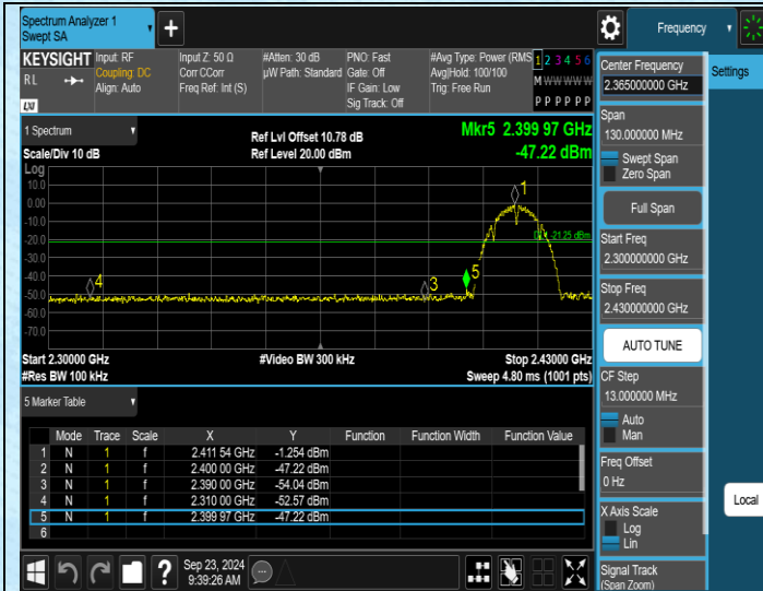
11B-Ant1-2412-PASS
