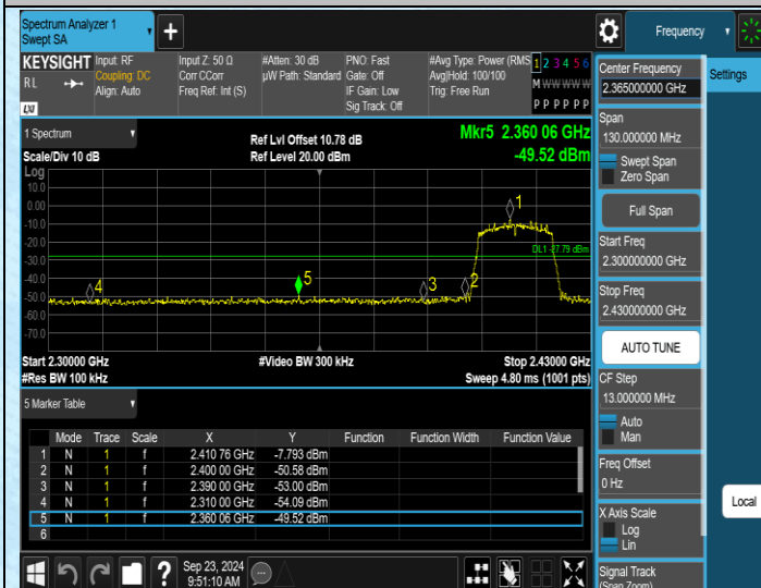
11N20SISO-Ant1-2412-PASS
