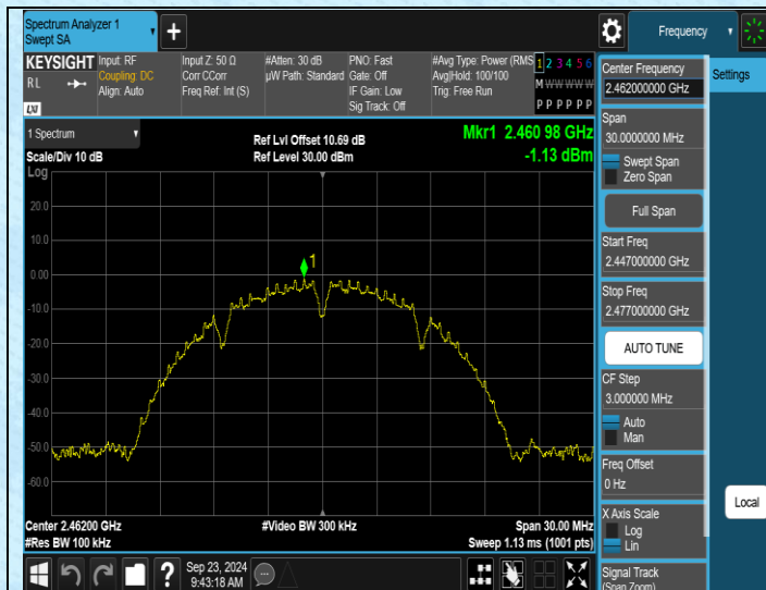
11B-Ant1-2462-0~Reference-PASS
