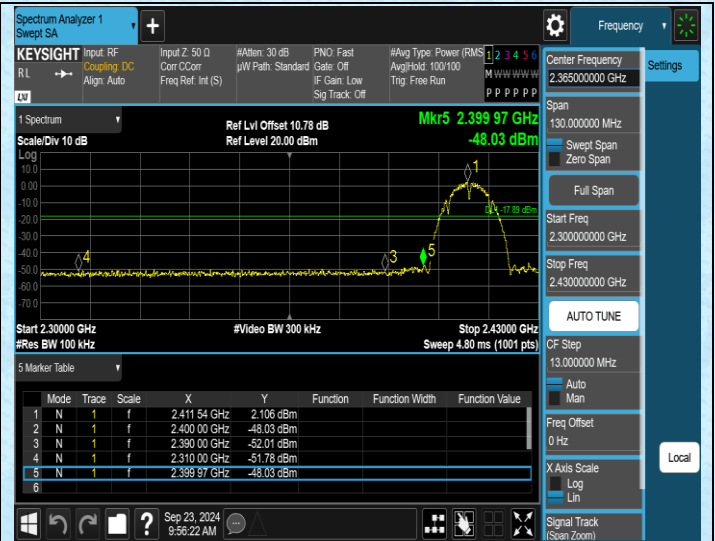
11B-Ant2-2412-PASS
