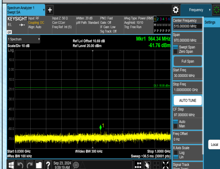
11B-Ant2-2462-30~1000-PASS
