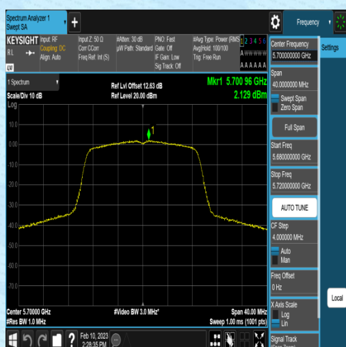
11AC20SISO-Ant2-5700-2.00-0.13-0.00-0.00
