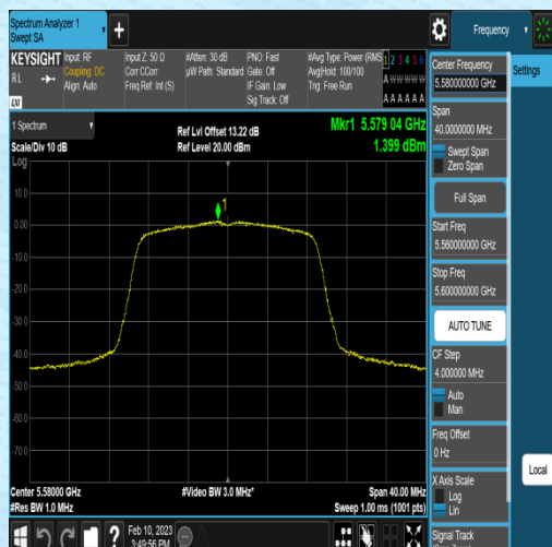
11N20MIMO-Ant1-5580-1.27-0.13-0.00-0.00
