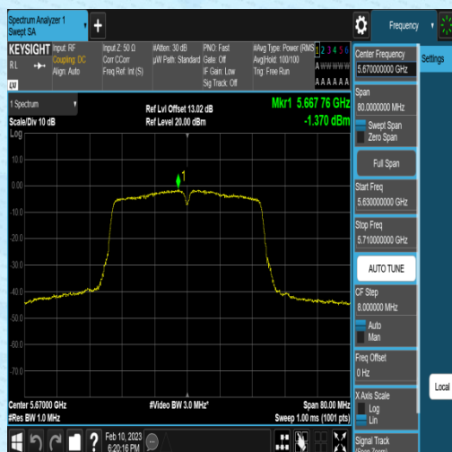
11AC40MIMO-Ant1-5670--1.84-0.47-0.00-0.00
