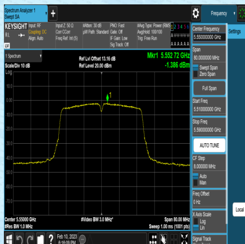
11AC40MIMO-Ant1-5550--1.97-0.58-0.00-0.00
