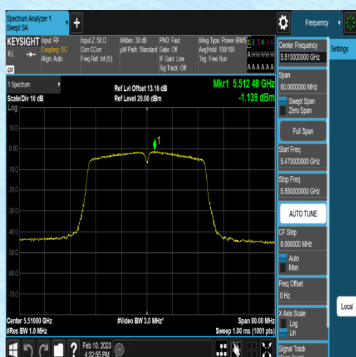
11N40MIMO-Ant1-5510--1.40-0.26-0.00-0.00
