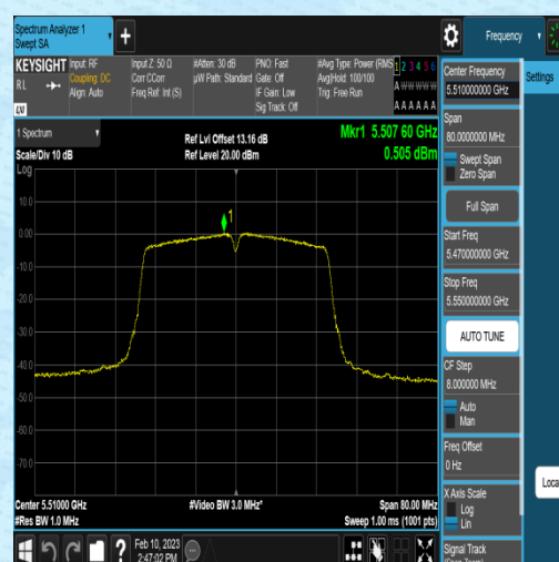
11AC40SISO-Ant2-5510-0.25-0.26-0.00-0.00
