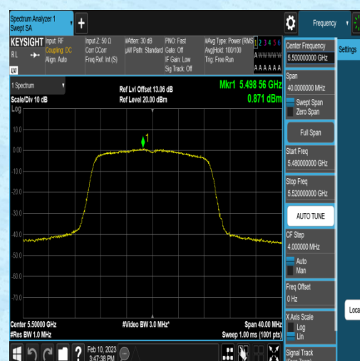
11N20MIMO-Ant2-5500-0.71-0.16-0.00-0.00
