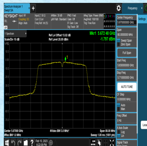
11AC40MIMO-Ant2-5670--2.27-0.47-0.00-0.00
