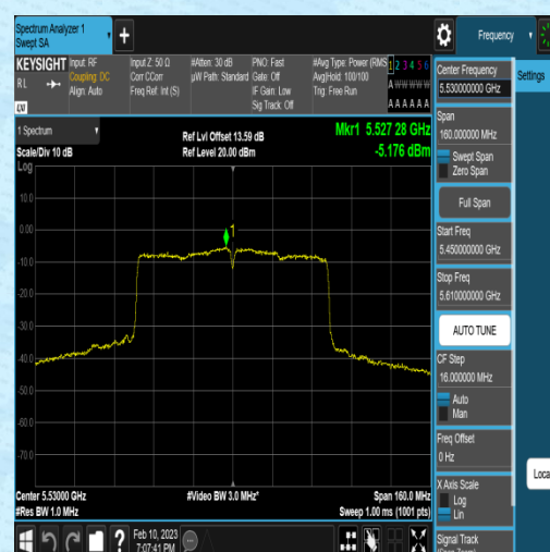
11AC80MIMO-Ant2-5530--6.01-0.83-0.00-0.00
