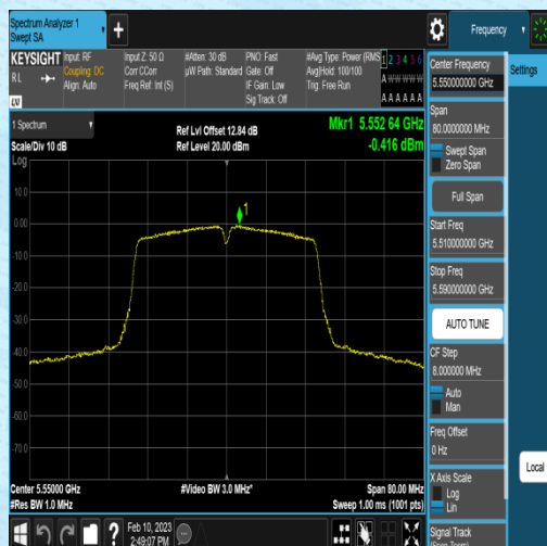
11AC40SISO-Ant2-5550--0.68-0.26-0.00-0.00
