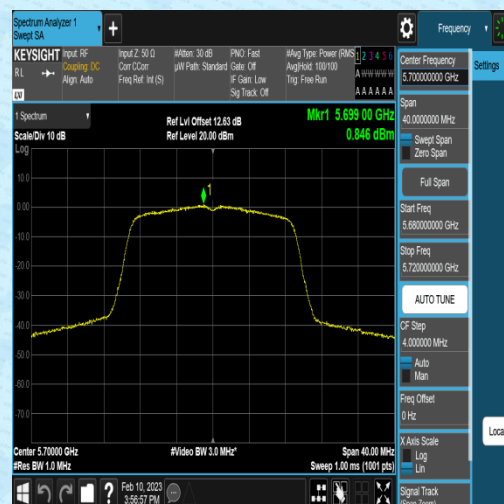
11N20MIMO-Ant2-5700-0.72-0.13-0.00-0.00
