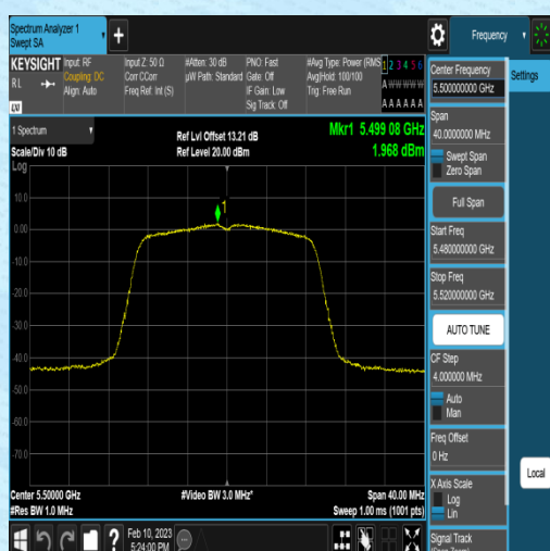
11AC20MIMO-Ant1-5500-1.66-0.31-0.00-0.00
