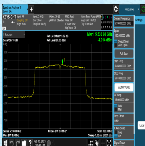
11AC80MIMO-Ant1-5530--5.07-1.06-0.00-0.00
