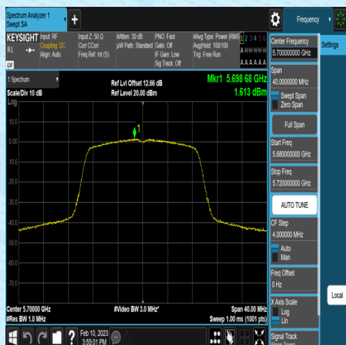
11N20MIMO-Ant1-5700-1.45-0.16-0.00-0.00
