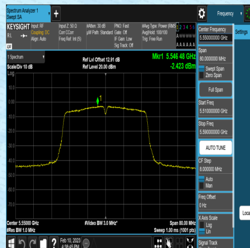
11N40MIMO-Ant2-5550--2.75-0.33-0.00-0.00
