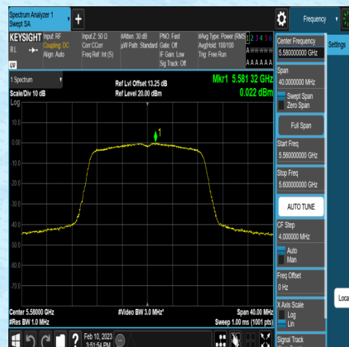
11N20MIMO-Ant2-5580--0.14-0.16-0.00-0.00
