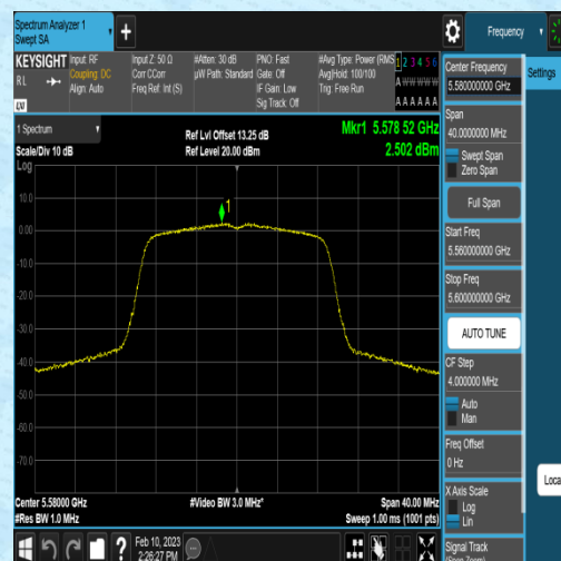
11AC20SISO-Ant2-5580-2.34-0.16-0.00-0.00
