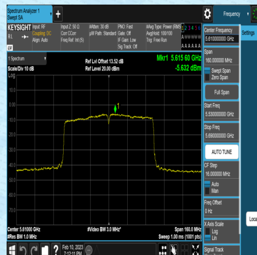
11AC80MIMO-Ant2-5610--6.46-0.83-0.00-0.00
