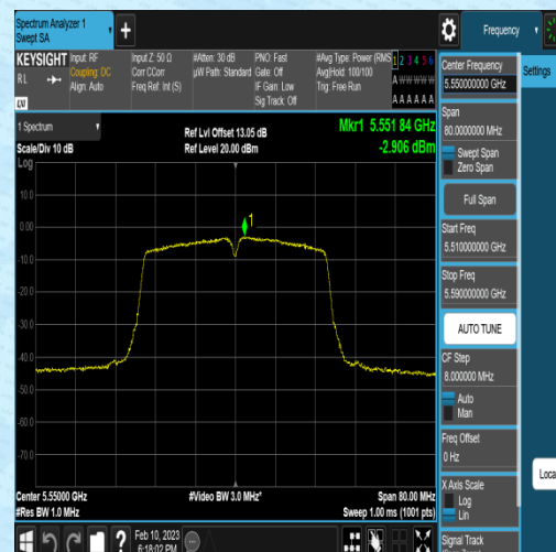
11AC40MIMO-Ant2-5550--3.38-0.47-0.00-0.00
