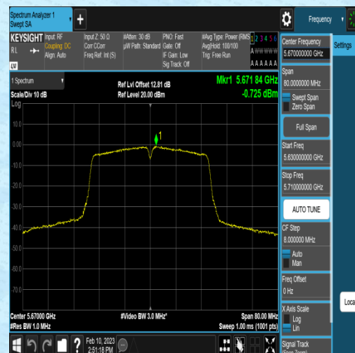
11AC40SISO-Ant2-5670--0.99-0.26-0.00-0.00
