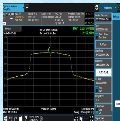
11N40MIMO-Ant2-5510--2.43-0.26-0.00-0.00
