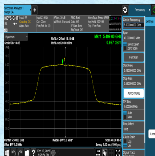
11AC20MIMO-Ant2-5500-0.72-0.25-0.00-0.00
