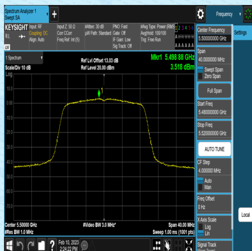
11AC20SISO-Ant2-5500-3.39-0.13-0.00-0.00
