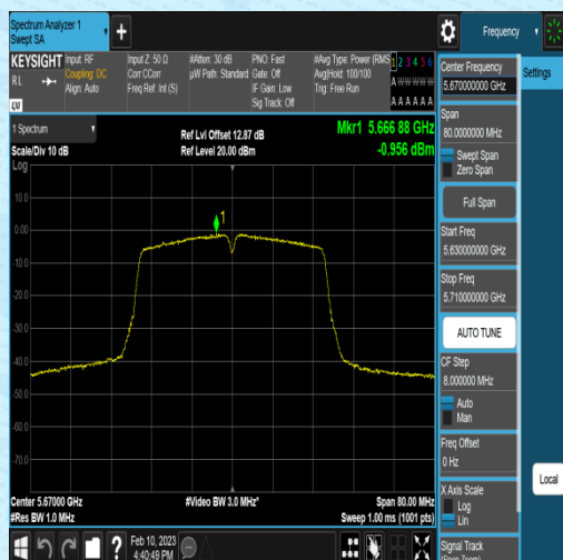
11N40MIMO-Ant1-5670--1.28-0.32-0.00-0.00
