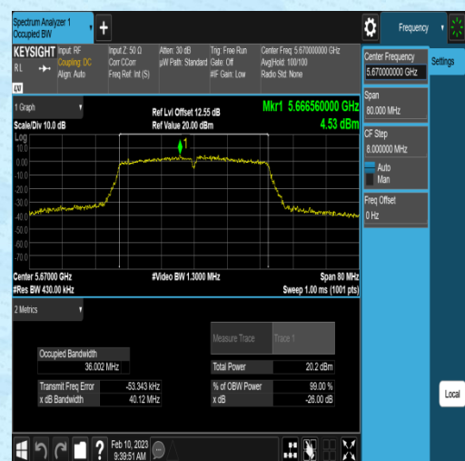
11AC40SISO-Ant1-5670
