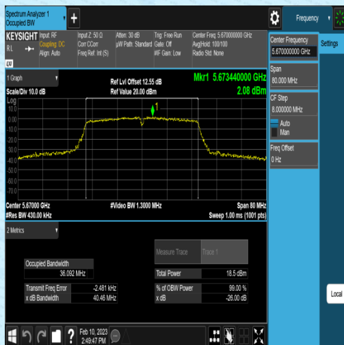
11AC40SISO-Ant2-5670
