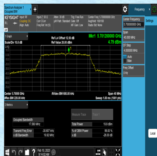
11AC20SISO-Ant1-5700
