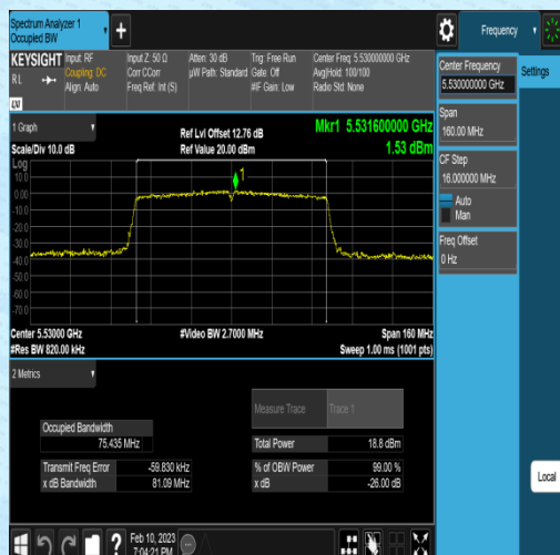
11AC80MIMO-Ant1-5530
