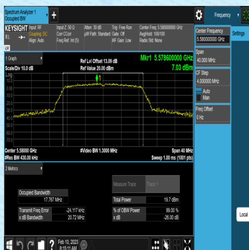
11N20SISO-Ant1-5580
