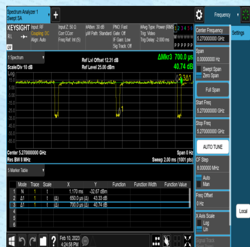
NTVN-11N40MIMO-Ant2-5270-0.65-0.70
