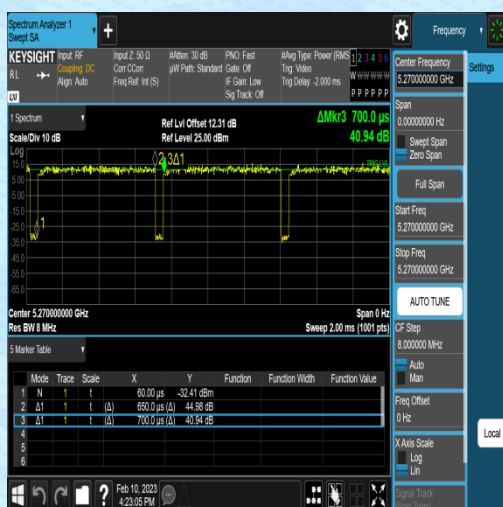
NTVN-11N40MIMO-Ant1-5270-0.65-0.70
