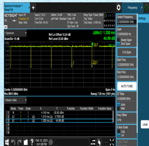
NTVN-11N20MIMO-Ant2-5320-1.31-1.35
