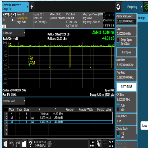
NTVN-11N20MIMO-Ant1-5280-1.30-1.34
