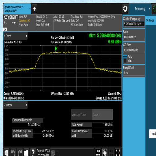
11N20SISO-Ant1-5260
