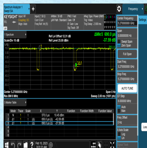
NTNV-11AC40SISO-Ant1-5270-0.65-0.69
