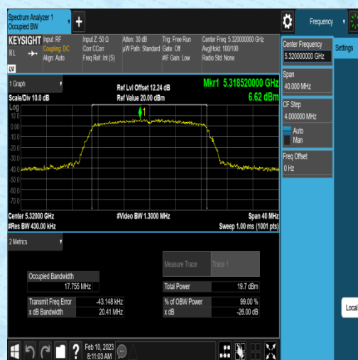
11N20SISO-Ant1-5320
