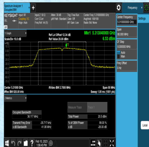
11N40SISO-Ant2-5310
