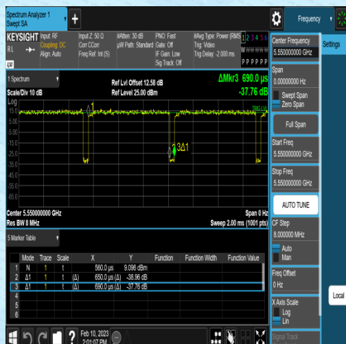
NTNV-11N40SISO-Ant2-5550-0.65-0.69
