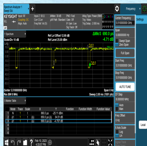
NTNV-11N40MIMO-Ant2-5510-0.65-0.69
