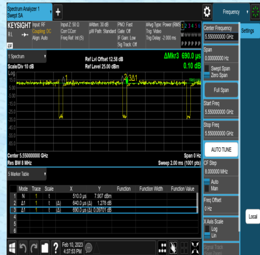
NTNV-11N40MIMO-Ant2-5550-0.64-0.69
