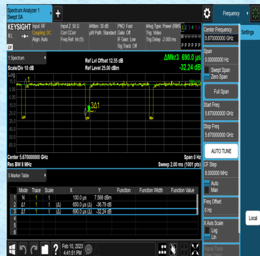
NTNV-11N40MIMO-Ant2-5670-0.65-0.69
