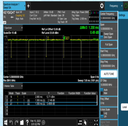
NTNV-11N20MIMO-Ant2-5580-1.30-1.35
