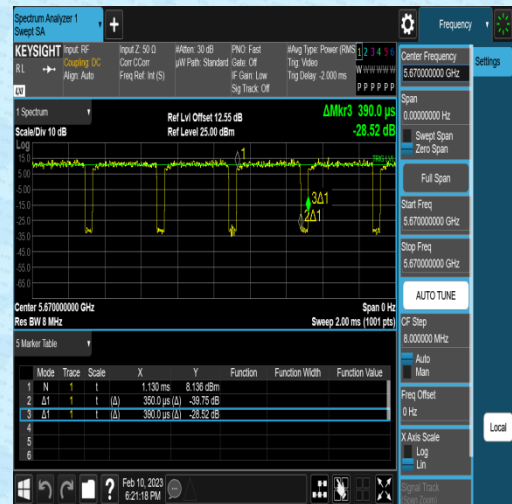
NTNV-11AC40MIMO-Ant2-5670-0.35-0.39
