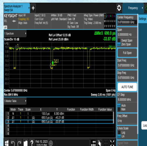
NTNV-11N40SISO-Ant2-5670-0.65-0.69
