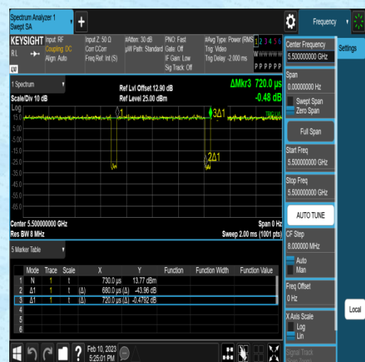
NTNV-11AC20MIMO-Ant2-5500-0.68-0.72
