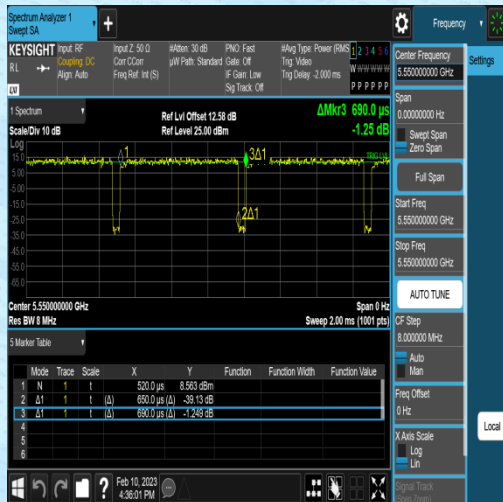
NTNV-11N40MIMO-Ant1-5550-0.65-0.69
