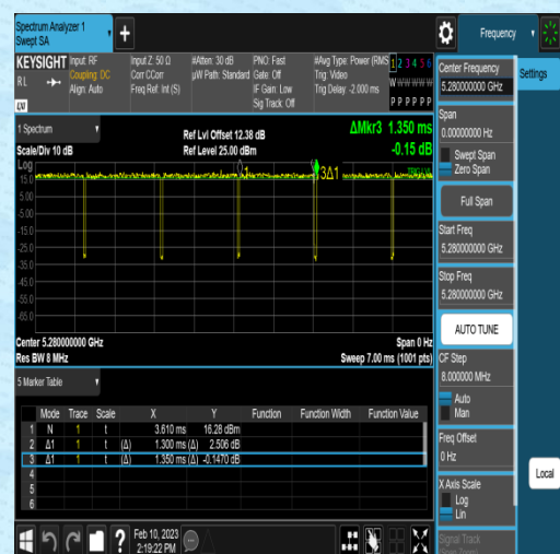
NTNV-11AC20SISO-Ant2-5280-1.30-1.35
