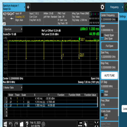
NTNV-11N20MIMO-Ant2-5320-1.31-1.35
