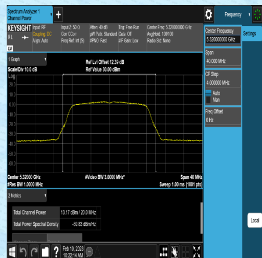
11A-Ant2-5320-NA----13.02-96.55-0.15
