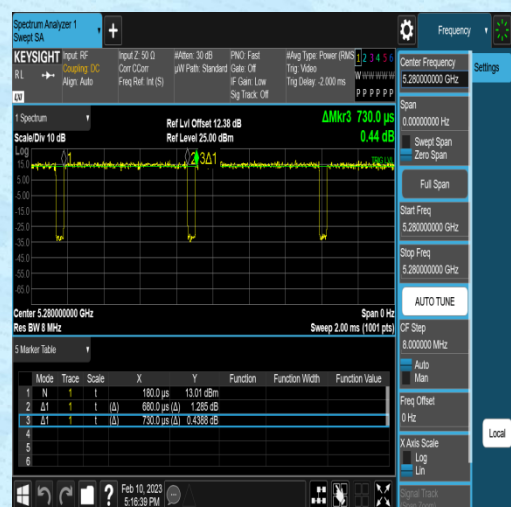
NTNV-11AC20MIMO-Ant2-5280-0.68-0.73
