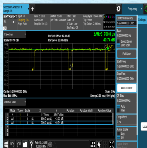
NTNV-11N40MIMO-Ant2-5270-0.65-0.70
