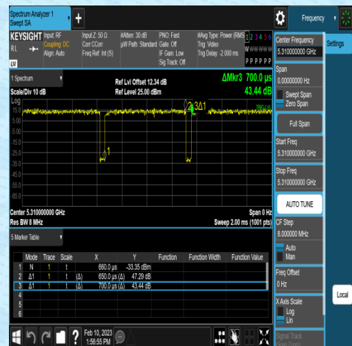
NTNV-11N40SISO-Ant2-5310-0.65-0.70
