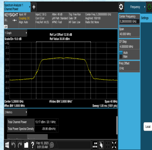
11A-Ant1-5280-NA----13.05-97.20-0.12
