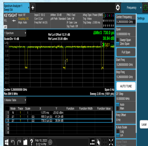
NTNV-11AC20MIMO-Ant2-5260-0.68-0.73
