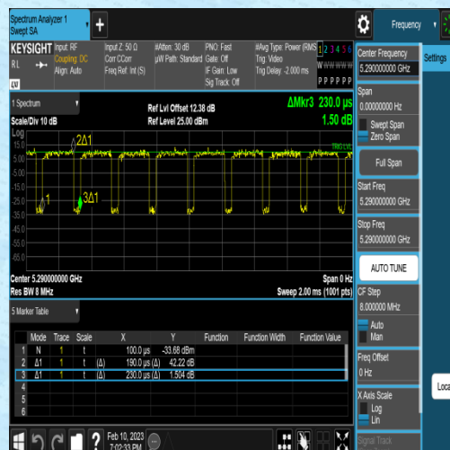
NTVN-11AC80MIMO-Ant2-5290-0.19-0.23
