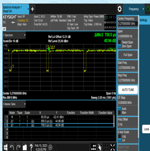
NTNV-11N40MIMO-Ant1-5270-0.65-0.70
