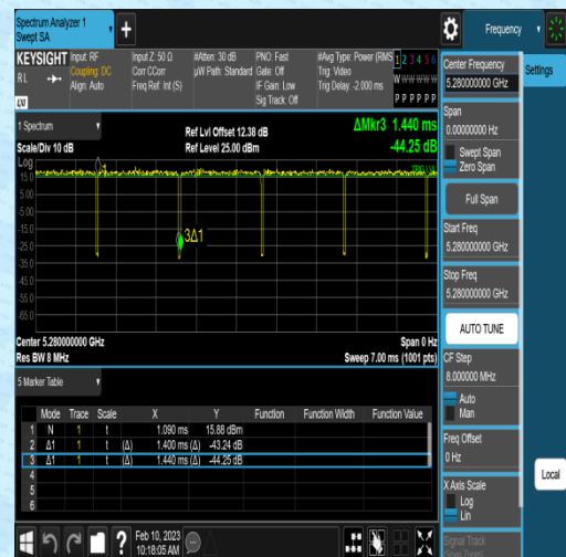
NTNV-11A-Ant2-5280-1.40-1.44
