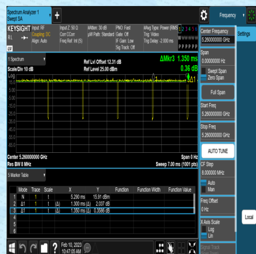
NTNV-11N20SISO-Ant2-5260-1.30-1.35
