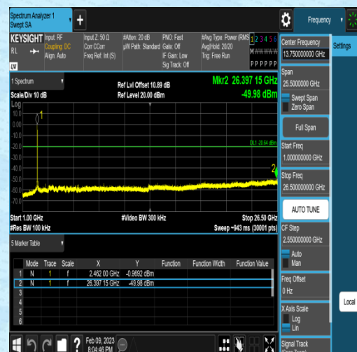
11G-Ant2-2462-1000~26500-0.64
