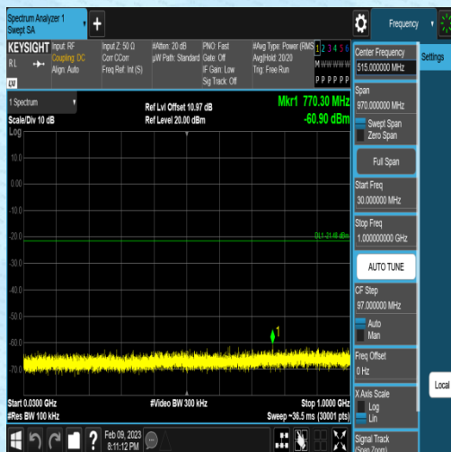
11N20SISO-Ant2-2437-30~1000--1.48
