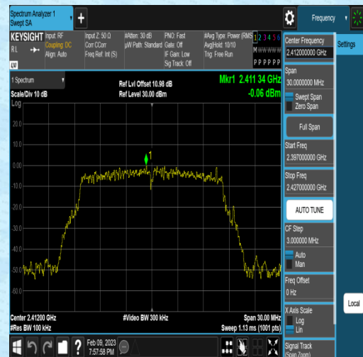
11G-Ant2-2412-Reference--0.06
