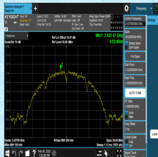
11B-Ant2-2437-Reference-4.52
