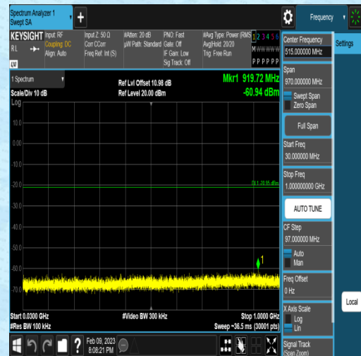
11N20SISO-Ant2-2412-30~1000--0.95
