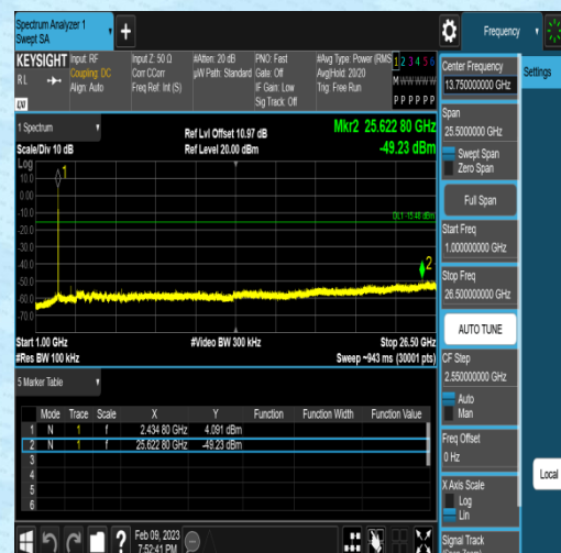
11B-Ant2-2437-1000~26500-4.52
