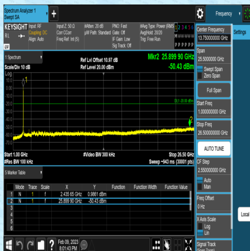
11G-Ant2-2437-1000~26500-0.00
