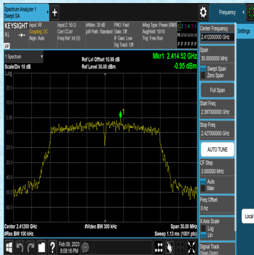
11N20SISO-Ant2-2412-Reference--0.95
