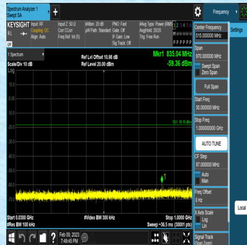
11B-Ant2-2412-30~1000-1.90
