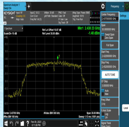
11N20SISO-Ant2-2437-Reference--1.48
