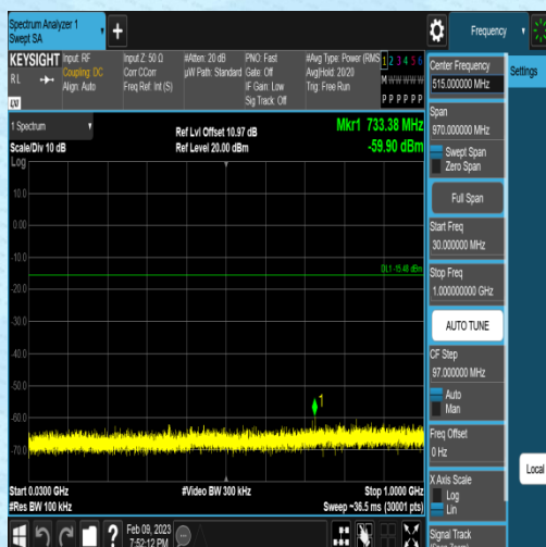
11B-Ant2-2437-30~1000-4.52
