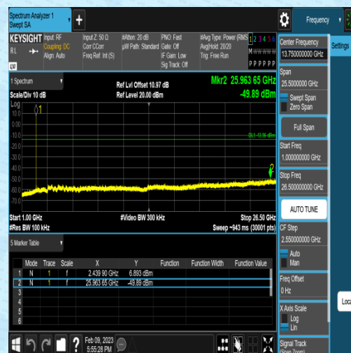
BLE_1M-Ant1-2440-1000~26500-6.04
