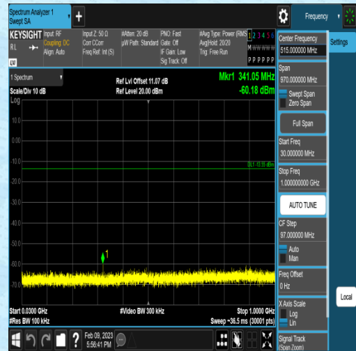
BLE_1M-Ant1-2480-30~1000-6.45
