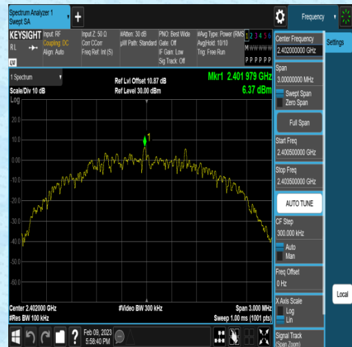
BLE_2M-Ant1-2402-Reference-6.37
