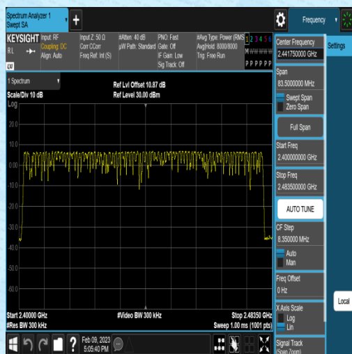
2DH5-Ant1-Hop
