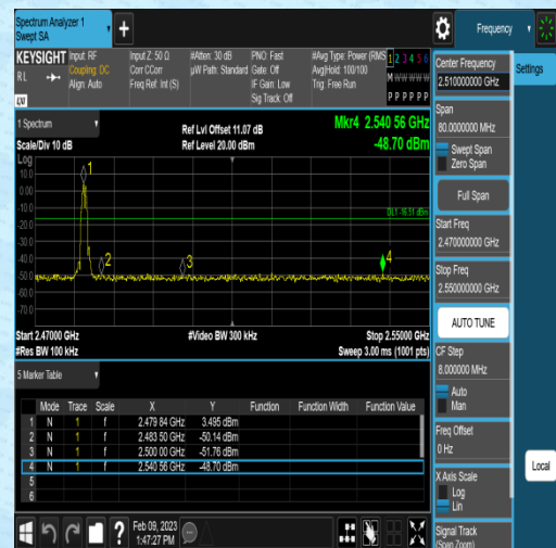
3DH5-Ant1-High-2480-3.50
