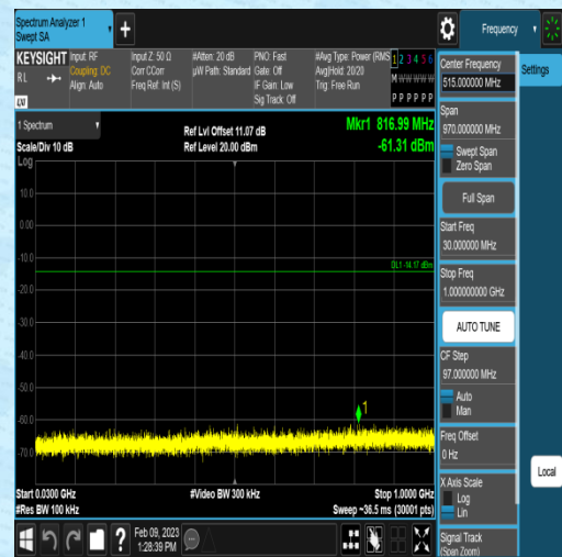
DH5-Ant1-2480-30~1000-5.83
