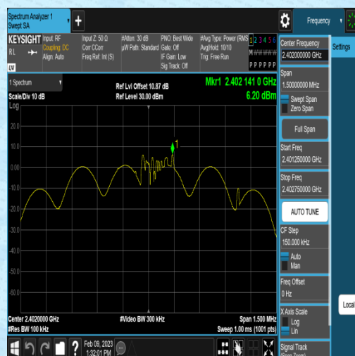
2DH5-Ant1-2402-Reference-6.20
