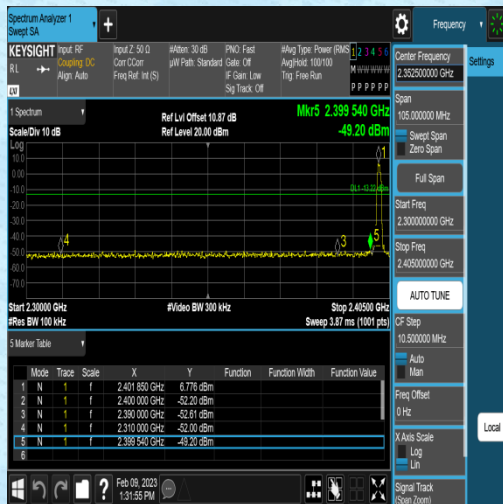
2DH5-Ant1-Low-2402-6.78
