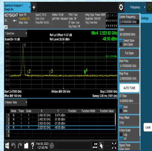
DH5-Ant1-High-2480-6.47
