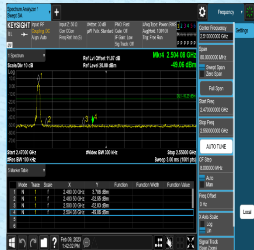
2DH5-Ant1-High-2480-3.71
