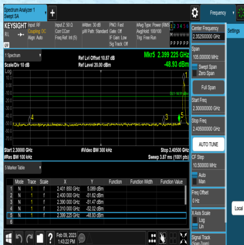
3DH5-Ant1-Low-2402-5.09
