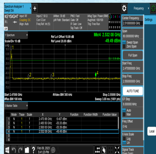
3DH5-Ant1-High-Hop_2480-6.41
