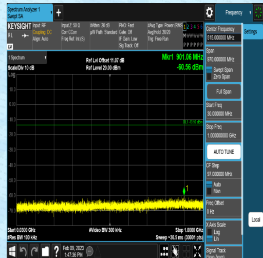
3DH5-Ant1-2480-30~1000-6.50
