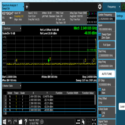
3DH5-Ant1-Low-Hop_2402-0.05
