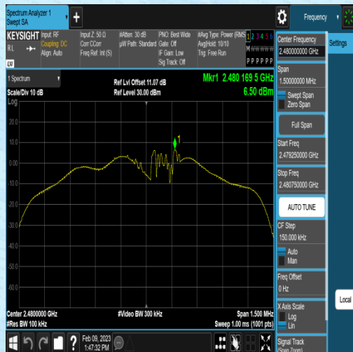
3DH5-Ant1-2480-Reference-6.50
