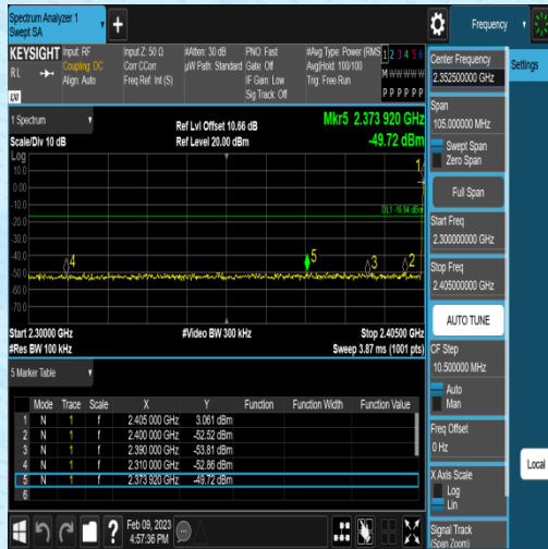
2DH5-Ant1-Low-Hop_2402-3.06
