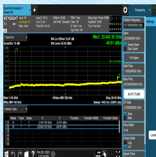
2DH5-Ant1-2402-1000~26500-6.20
