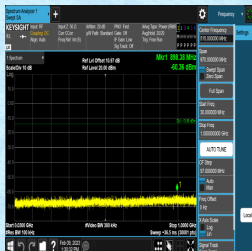
DH5-Ant1-2441-30~1000-6.14
