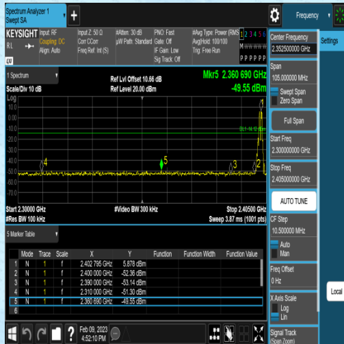
DH5-Ant1-Low-Hop_2402-5.88
