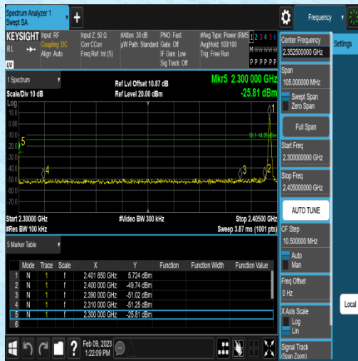
DH5-Ant1-Low-2402-5.72
