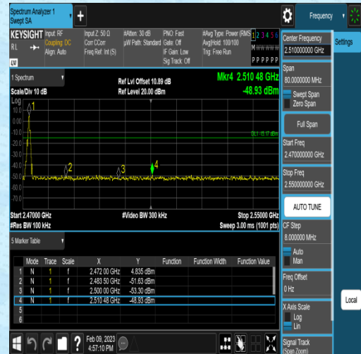
DH5-Ant1-High-Hop_2480-4.84
