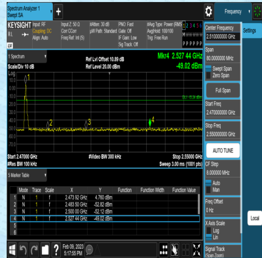
2DH5-Ant1-High-Hop_2480-4.76
