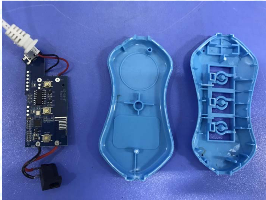
Model: XHBT02 Photo 2 Internal of EUT
